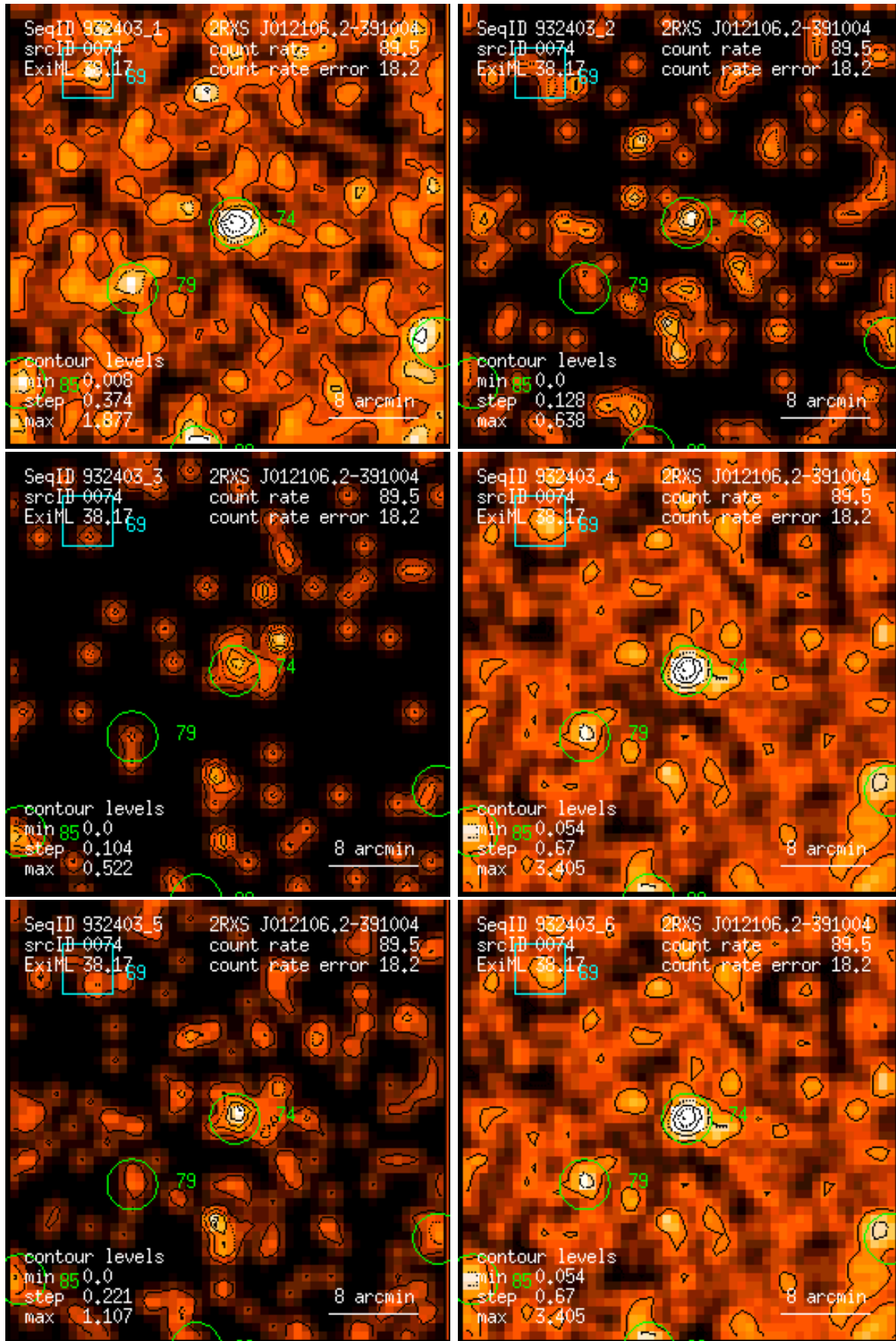
Figure 74: RASS 932403: detection 0074: band rate images, Gaussian filter: (1) PSPC channels 11 – 41, (2) 52 – 90, (3) 91 – 201, (4) 11 – 235, (5) 52 – 201, (6) 11 – 201. Broad band rates in counts/ks. Band rate contour levels in counts/ks/arcmin 2 .
