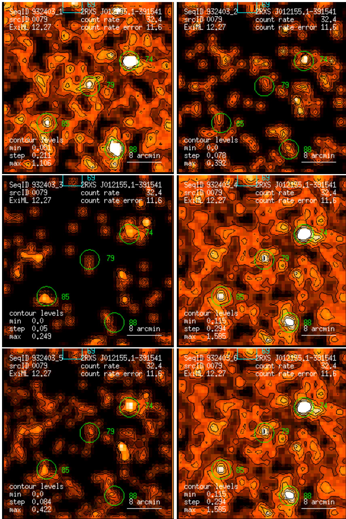
Figure 79: RASS 932403: detection 0079: band rate images, Gaussian filter: (1) PSPC channels 11 – 41, (2) 52 – 90, (3) 91 – 201, (4) 11 – 235, (5) 52 – 201, (6) 11 – 201. Broad band rates in counts/ks. Band rate contour levels in counts/ks/arcmin 2 .
