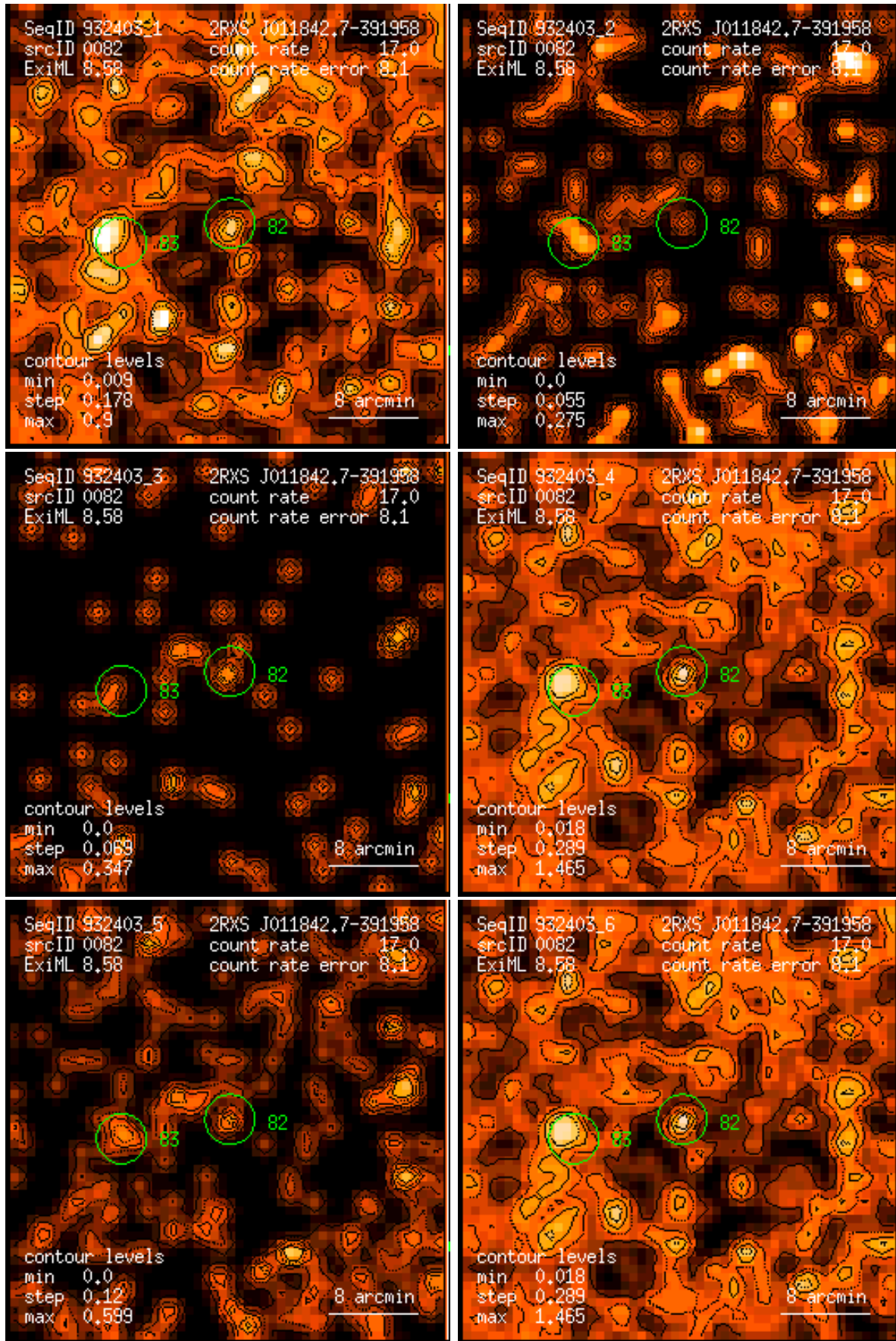
Figure 82: RASS 932403: detection 0082: band rate images, Gaussian filter: (1) PSPC channels 11 – 41, (2) 52 – 90, (3) 91 – 201, (4) 11 – 235, (5) 52 – 201, (6) 11 – 201. Broad band rates in counts/ks. Band rate contour levels in counts/ks/arcmin 2 .
