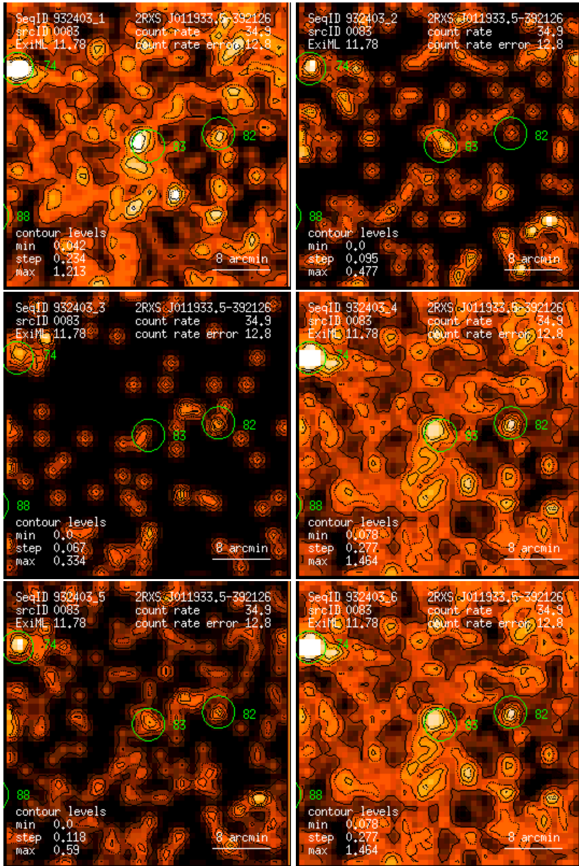
Figure 83: RASS 932403: detection 0083: band rate images, Gaussian filter: (1) PSPC channels 11 – 41, (2) 52 – 90, (3) 91 – 201, (4) 11 – 235, (5) 52 – 201, (6) 11 – 201. Broad band rates in counts/ks. Band rate contour levels in counts/ks/arcmin 2 .
