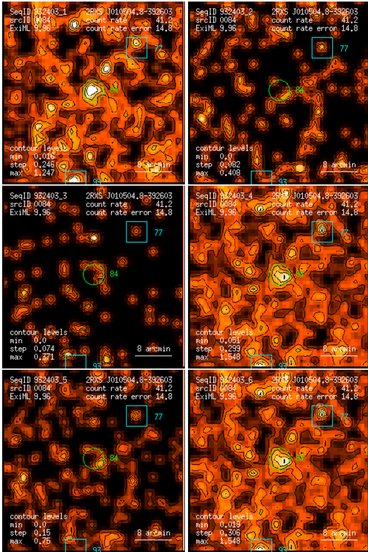
Figure 84: RASS 932403: detection 0084: band rate images, Gaussian filter: (1) PSPC channels 11 – 41, (2) 52 – 90, (3) 91 – 201, (4) 11 – 235, (5) 52 – 201, (6) 11 – 201. Broad band rates in counts/ks. Band rate contour levels in counts/ks/arcmin 2 .
