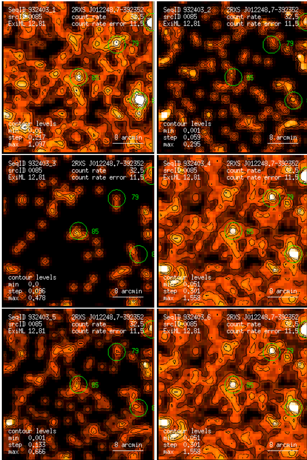
Figure 85: RASS 932403: detection 0085: band rate images, Gaussian filter: (1) PSPC channels 11 – 41, (2) 52 – 90, (3) 91 – 201, (4) 11 – 235, (5) 52 – 201, (6) 11 – 201. Broad band rates in counts/ks. Band rate contour levels in counts/ks/arcmin 2 .
