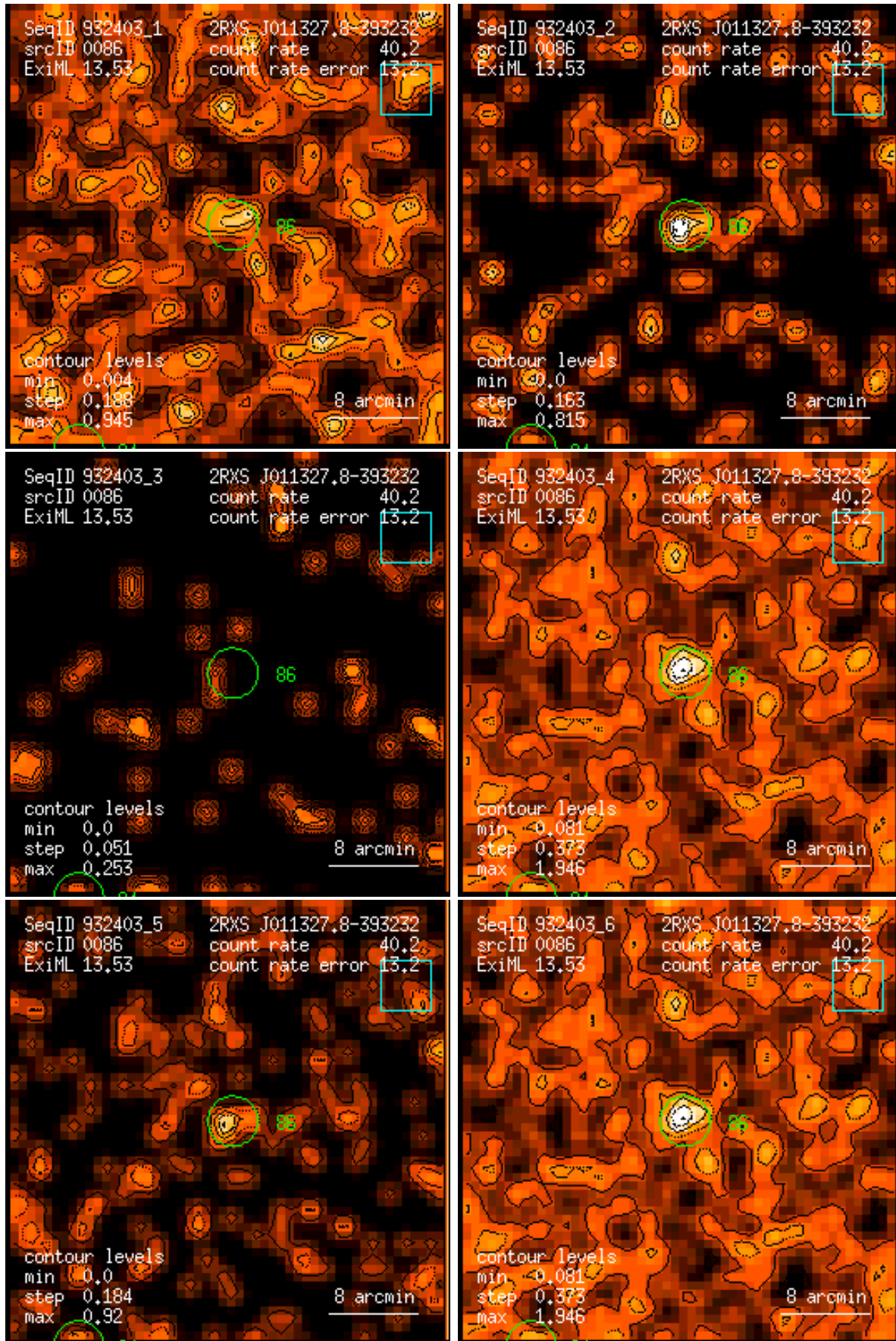
Figure 86: RASS 932403: detection 0086: band rate images, Gaussian filter: (1) PSPC channels 11 – 41, (2) 52 – 90, (3) 91 – 201, (4) 11 – 235, (5) 52 – 201, (6) 11 – 201. Broad band rates in counts/ks. Band rate contour levels in counts/ks/arcmin 2 .
