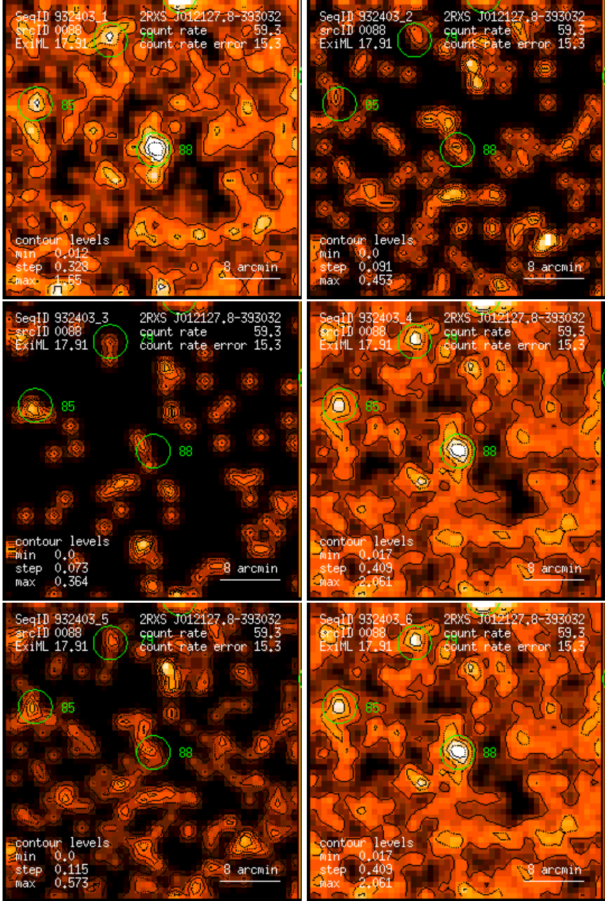
Figure 88: RASS 932403: detection 0088: band rate images, Gaussian filter: (1) PSPC channels 11 – 41, (2) 52 – 90, (3) 91 – 201, (4) 11 – 235, (5) 52 – 201, (6) 11 – 201. Broad band rates in counts/ks. Band rate contour levels in counts/ks/arcmin 2 .
