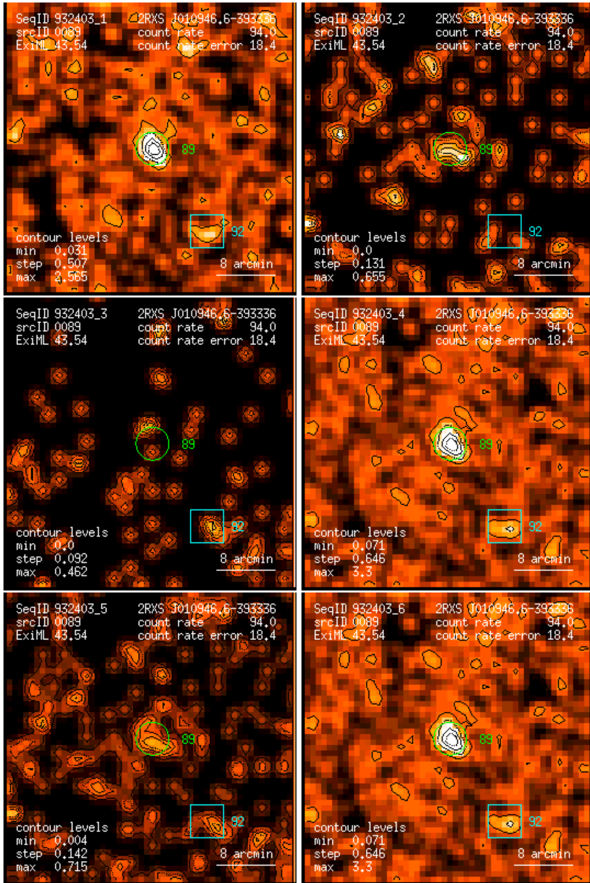
Figure 89: RASS 932403: detection 0089: band rate images, Gaussian filter: (1) PSPC channels 11 – 41, (2) 52 – 90, (3) 91 – 201, (4) 11 – 235, (5) 52 – 201, (6) 11 – 201. Broad band rates in counts/ks. Band rate contour levels in counts/ks/arcmin 2 .
