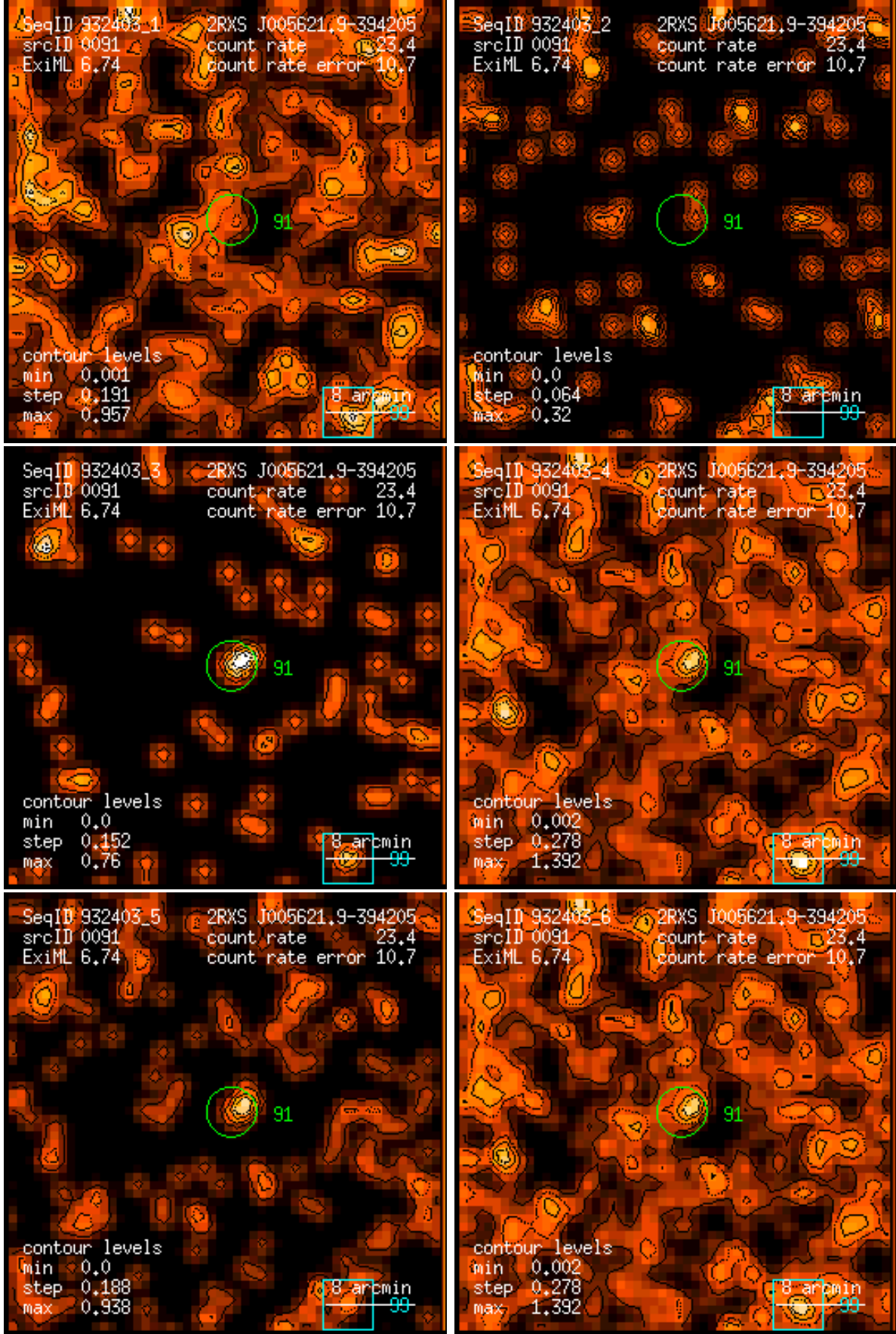
Figure 91: RASS 932403: detection 0091: band rate images, Gaussian filter: (1) PSPC channels 11 – 41, (2) 52 – 90, (3) 91 – 201, (4) 11 – 235, (5) 52 – 201, (6) 11 – 201. Broad band rates in counts/ks. Band rate contour levels in counts/ks/arcmin 2 .
