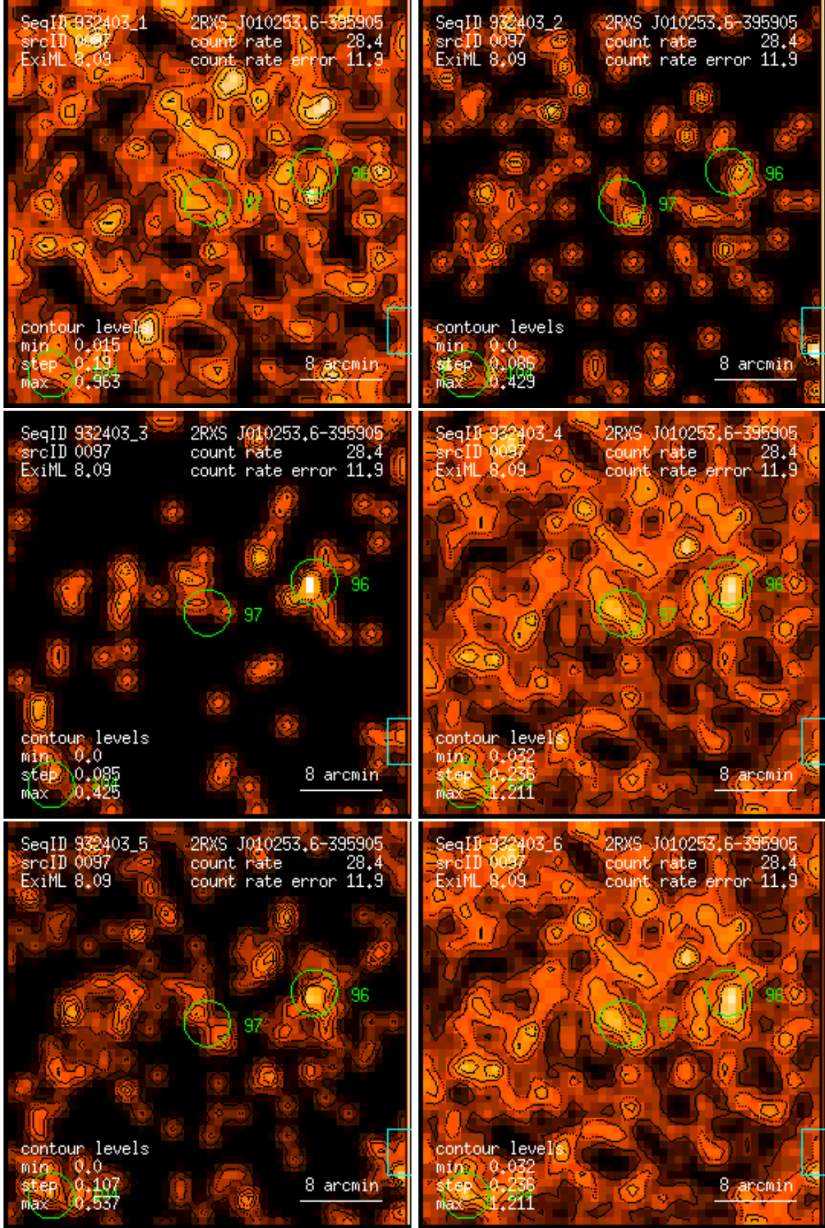
Figure 97: RASS 932403: detection 0097: band rate images, Gaussian filter: (1) PSPC channels 11 – 41, (2) 52 – 90, (3) 91 – 201, (4) 11 – 235, (5) 52 – 201, (6) 11 – 201. Broad band rates in counts/ks. Band rate contour levels in counts/ks/arcmin 2 .
