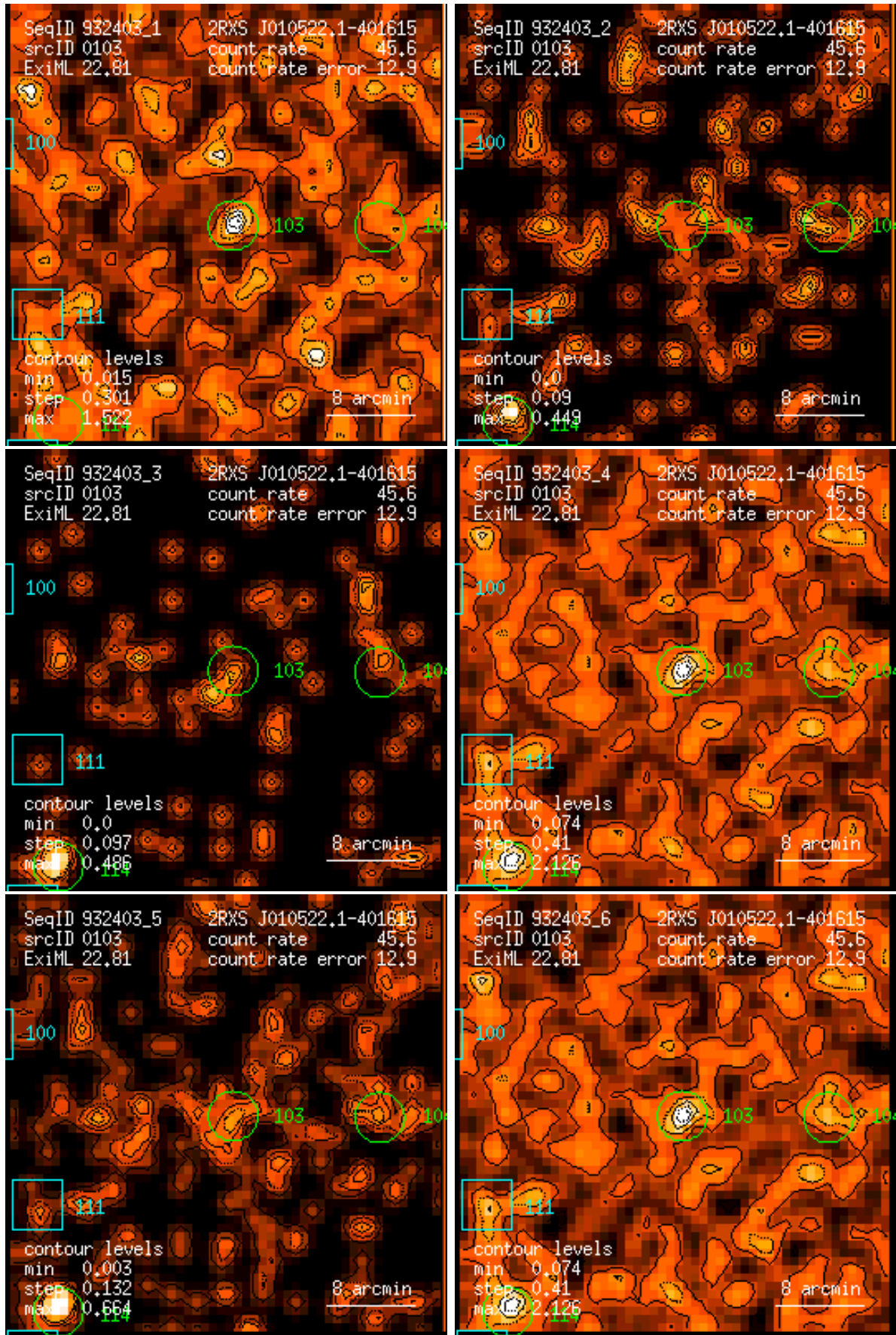
Figure 103: RASS 932403: detection 0103: band rate images, Gaussian filter: (1) PSPC channels 11 – 41, (2) 52 – 90, (3) 91 – 201, (4) 11 – 235, (5) 52 – 201, (6) 11 – 201. Broad band rates in counts/ks. Band rate contour levels in counts/ks/arcmin 2 .
