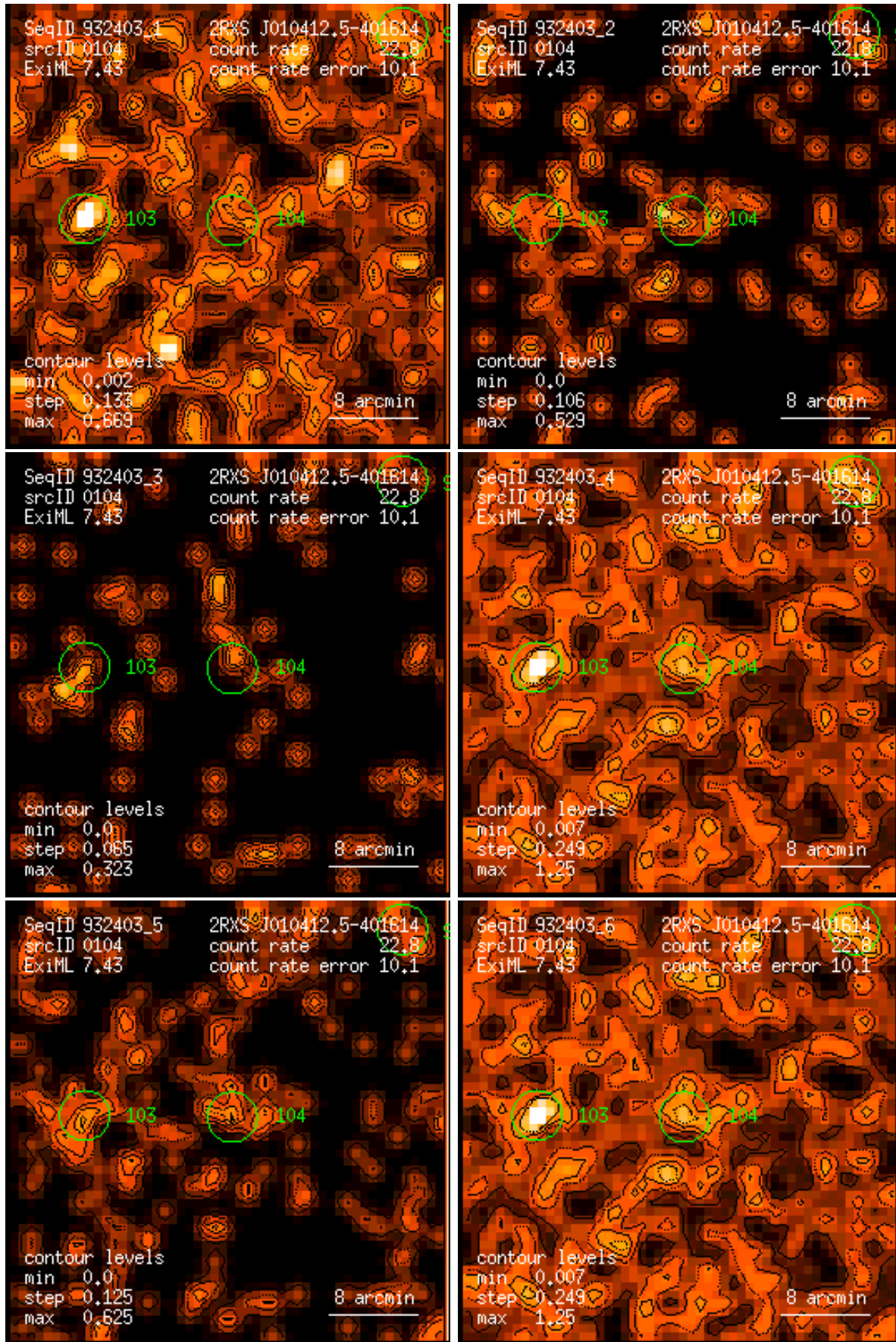
Figure 104: RASS 932403: detection 0104: band rate images, Gaussian filter: (1) PSPC channels 11 – 41, (2) 52 – 90, (3) 91 – 201, (4) 11 – 235, (5) 52 – 201, (6) 11 – 201. Broad band rates in counts/ks. Band rate contour levels in counts/ks/arcmin 2 .
