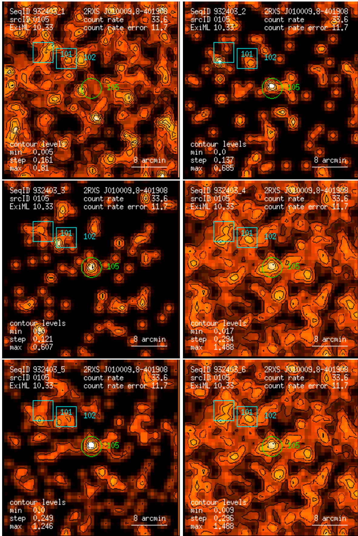
Figure 105: RASS 932403: detection 0105: band rate images, Gaussian filter: (1) PSPC channels 11 – 41, (2) 52 – 90, (3) 91 – 201, (4) 11 – 235, (5) 52 – 201, (6) 11 – 201. Broad band rates in counts/ks. Band rate contour levels in counts/ks/arcmin 2 .
