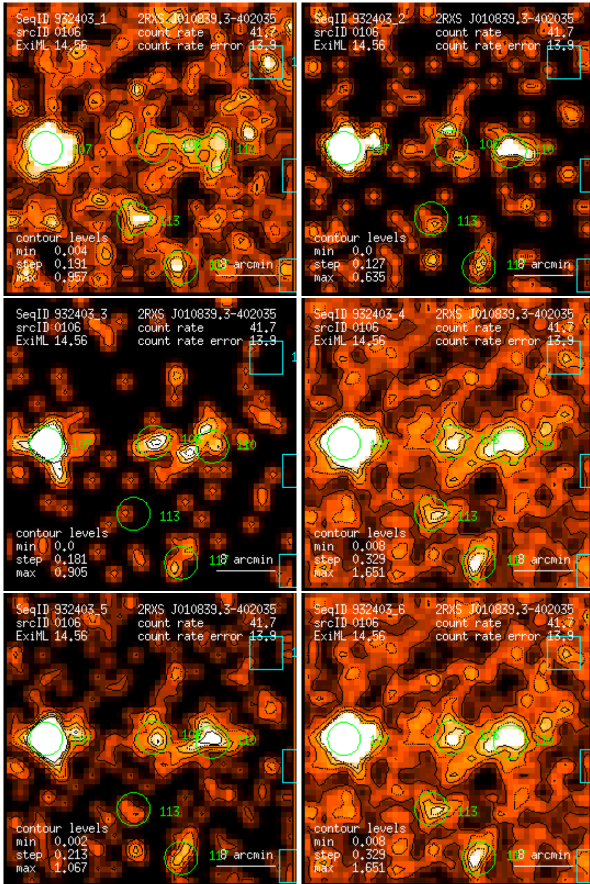
Figure 106: RASS 932403: detection 0106: band rate images, Gaussian filter: (1) PSPC channels 11 – 41, (2) 52 – 90, (3) 91 – 201, (4) 11 – 235, (5) 52 – 201, (6) 11 – 201. Broad band rates in counts/ks. Band rate contour levels in counts/ks/arcmin 2 .
