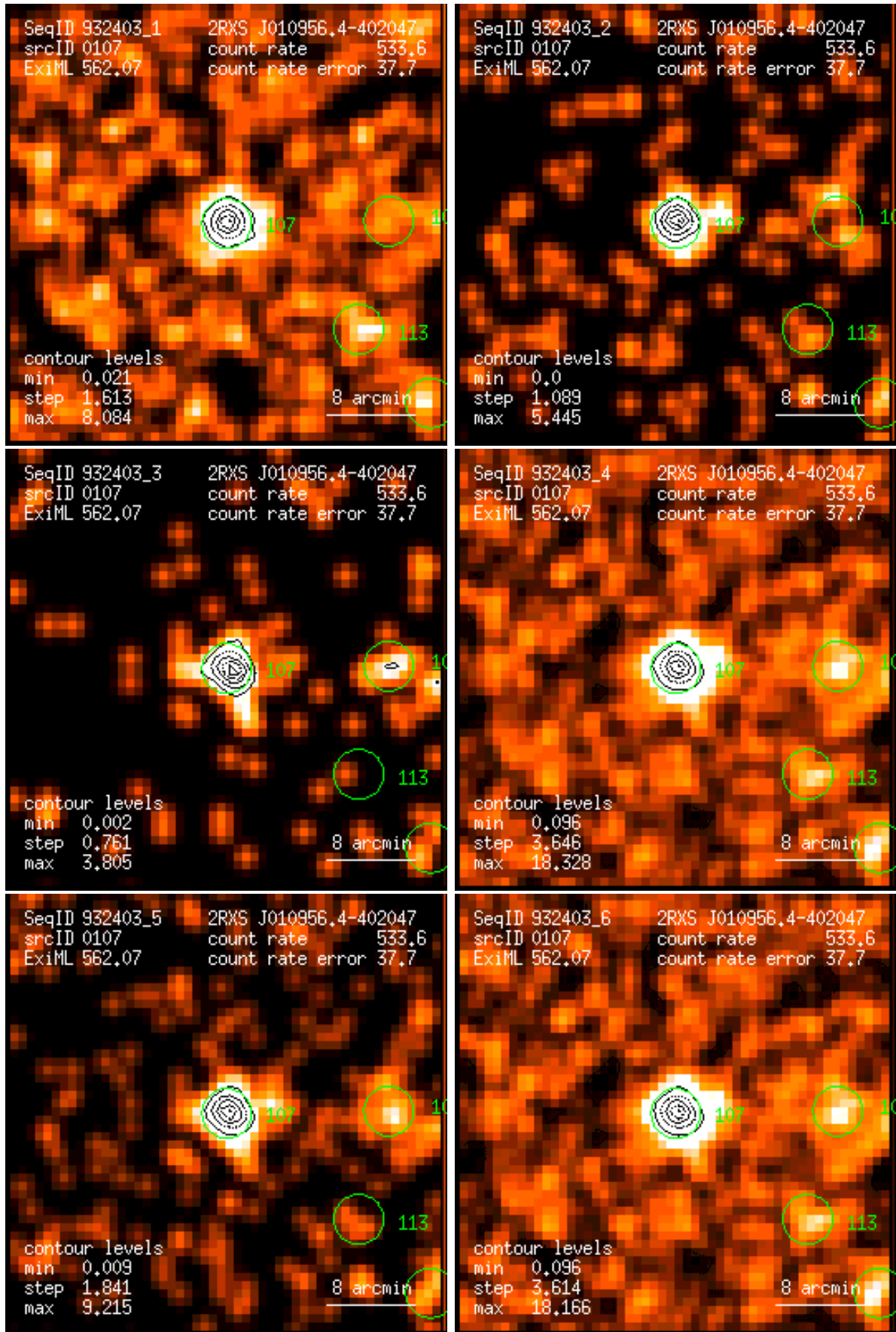
Figure 107: RASS 932403: detection 0107: band rate images, Gaussian filter: (1) PSPC channels 11 – 41, (2) 52 – 90, (3) 91 – 201, (4) 11 – 235, (5) 52 – 201, (6) 11 – 201. Broad band rates in counts/ks. Band rate contour levels in counts/ks/arcmin 2 .
