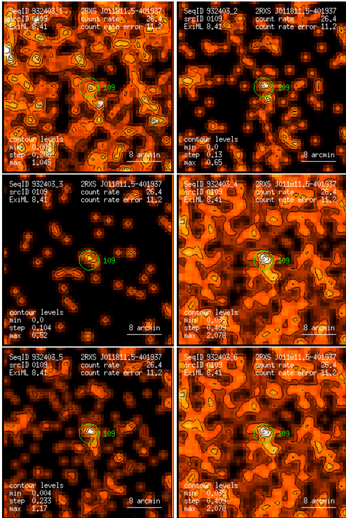
Figure 109: RASS 932403: detection 0109: band rate images, Gaussian filter: (1) PSPC channels 11 – 41, (2) 52 – 90, (3) 91 – 201, (4) 11 – 235, (5) 52 – 201, (6) 11 – 201. Broad band rates in counts/ks. Band rate contour levels in counts/ks/arcmin 2 .
