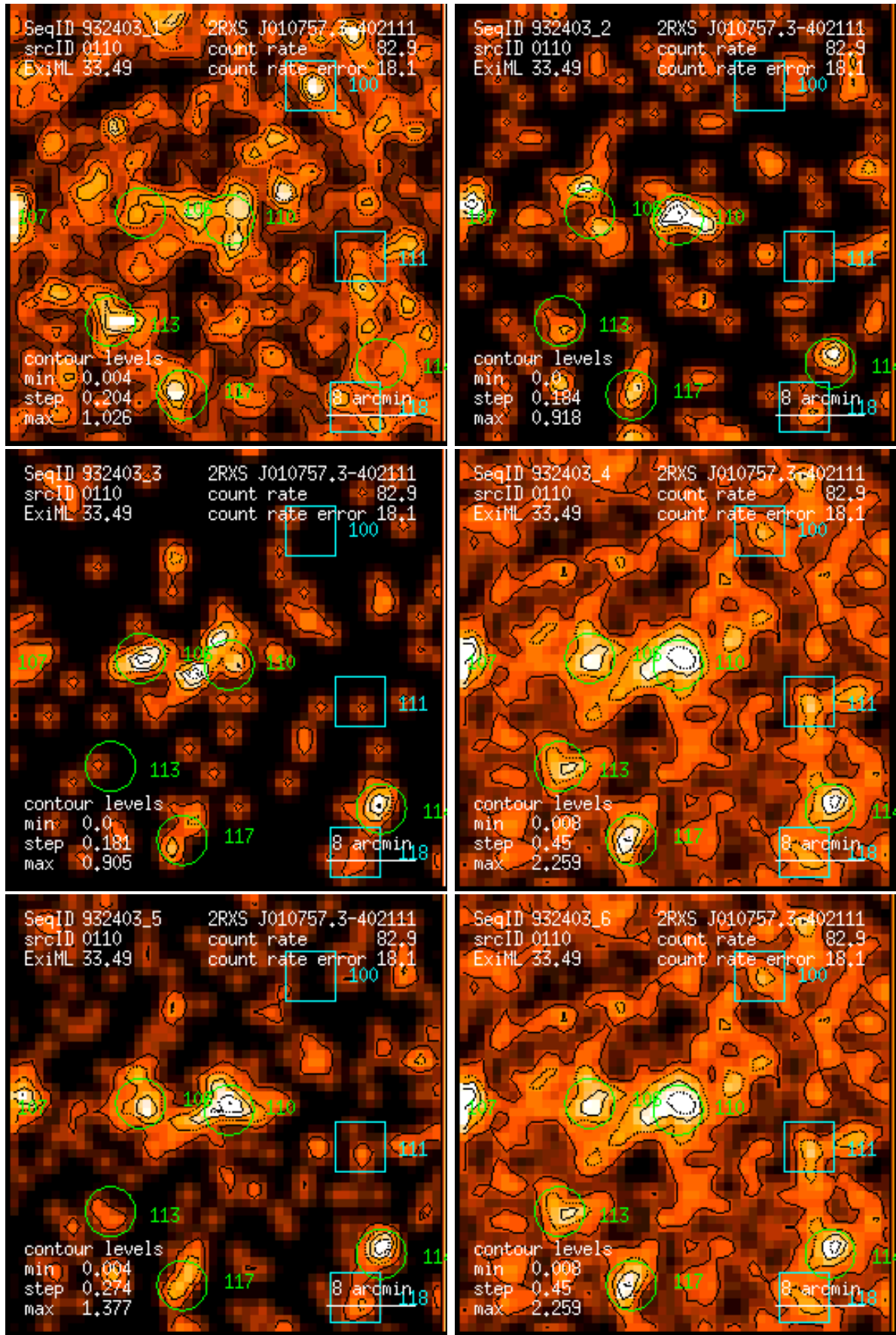
Figure 110: RASS 932403: detection 0110: band rate images, Gaussian filter: (1) PSPC channels 11 – 41, (2) 52 – 90, (3) 91 – 201, (4) 11 – 235, (5) 52 – 201, (6) 11 – 201. Broad band rates in counts/ks. Band rate contour levels in counts/ks/arcmin 2 .
