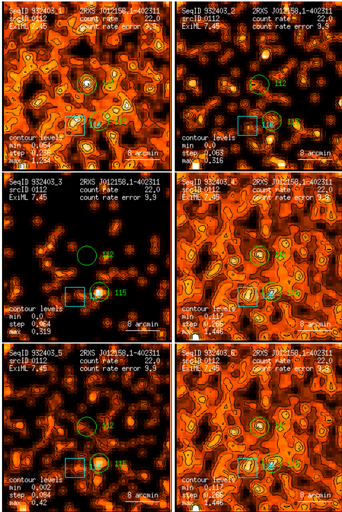
Figure 112: RASS 932403: detection 0112: band rate images, Gaussian filter: (1) PSPC channels 11 – 41, (2) 52 – 90, (3) 91 – 201, (4) 11 – 235, (5) 52 – 201, (6) 11 – 201. Broad band rates in counts/ks. Band rate contour levels in counts/ks/arcmin 2 .
