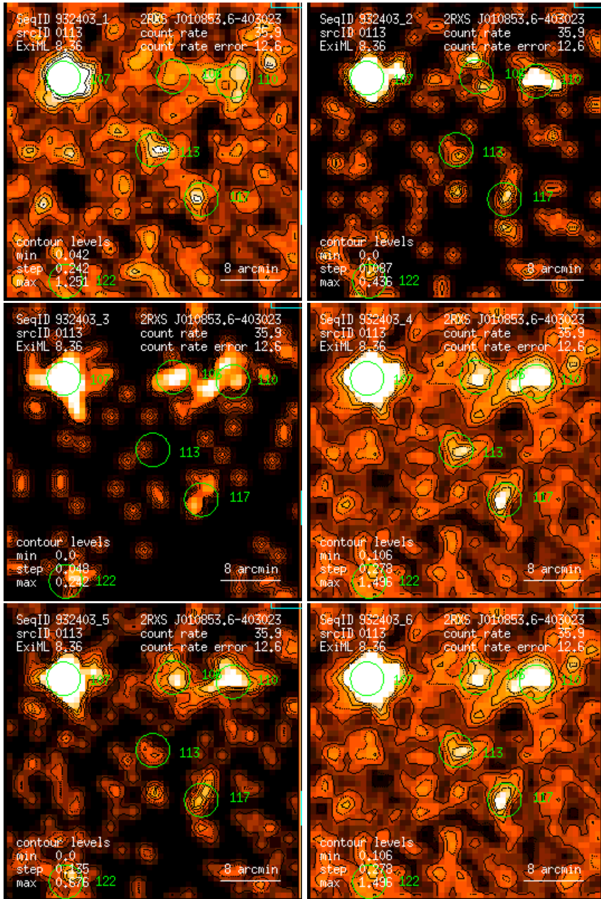
Figure 113: RASS 932403: detection 0113: band rate images, Gaussian filter: (1) PSPC channels 11 – 41, (2) 52 – 90, (3) 91 – 201, (4) 11 – 235, (5) 52 – 201, (6) 11 – 201. Broad band rates in counts/ks. Band rate contour levels in counts/ks/arcmin 2 .
