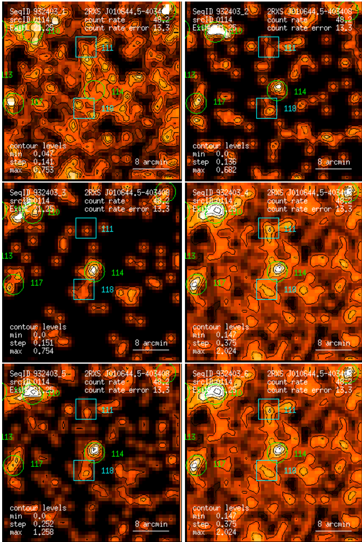
Figure 114: RASS 932403: detection 0114: band rate images, Gaussian filter: (1) PSPC channels 11 – 41, (2) 52 – 90, (3) 91 – 201, (4) 11 – 235, (5) 52 – 201, (6) 11 – 201. Broad band rates in counts/ks. Band rate contour levels in counts/ks/arcmin 2 .
