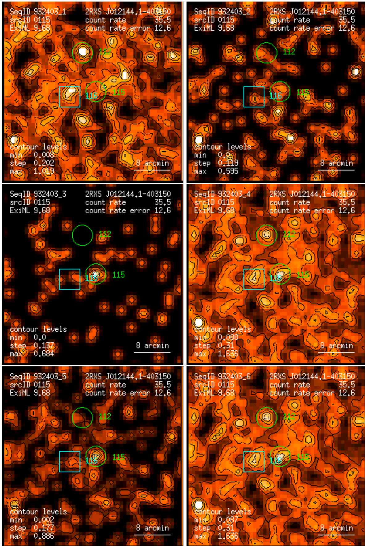
Figure 115: RASS 932403: detection 0115: band rate images, Gaussian filter: (1) PSPC channels 11 – 41, (2) 52 – 90, (3) 91 – 201, (4) 11 – 235, (5) 52 – 201, (6) 11 – 201. Broad band rates in counts/ks. Band rate contour levels in counts/ks/arcmin 2 .
