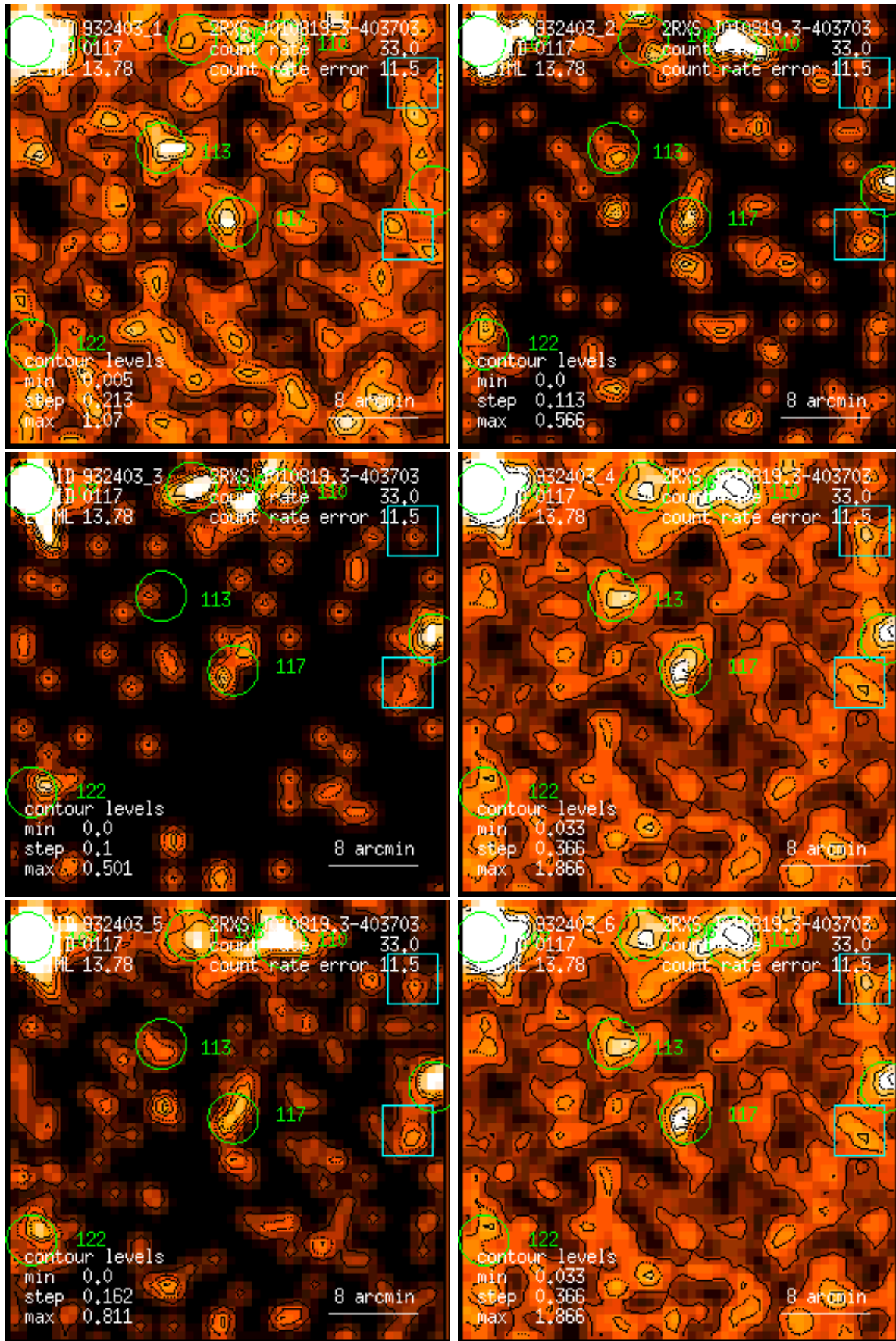
Figure 117: RASS 932403: detection 0117: band rate images, Gaussian filter: (1) PSPC channels 11 – 41, (2) 52 – 90, (3) 91 – 201, (4) 11 – 235, (5) 52 – 201, (6) 11 – 201. Broad band rates in counts/ks. Band rate contour levels in counts/ks/arcmin 2 .
