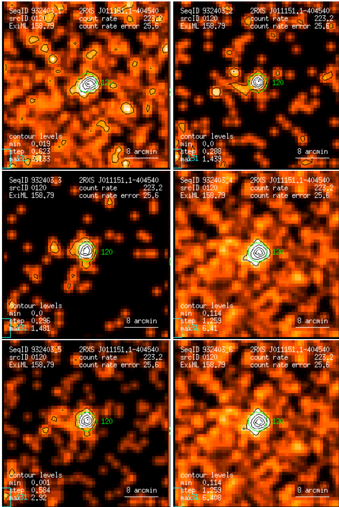
Figure 120: RASS 932403: detection 0120: band rate images, Gaussian filter: (1) PSPC channels 11 – 41, (2) 52 – 90, (3) 91 – 201, (4) 11 – 235, (5) 52 – 201, (6) 11 – 201. Broad band rates in counts/ks. Band rate contour levels in counts/ks/arcmin 2 .
