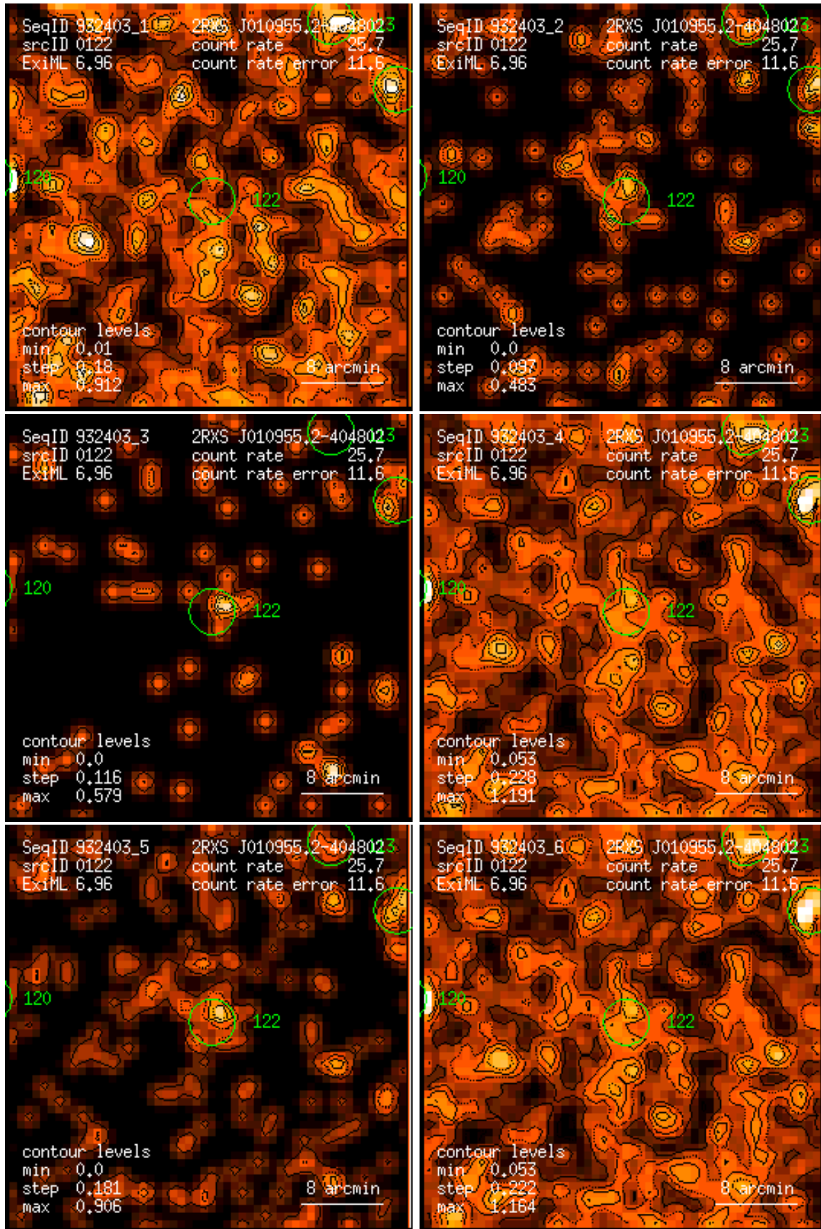
Figure 122: RASS 932403: detection 0122: band rate images, Gaussian filter: (1) PSPC channels 11 – 41, (2) 52 – 90, (3) 91 – 201, (4) 11 – 235, (5) 52 – 201, (6) 11 – 201. Broad band rates in counts/ks. Band rate contour levels in counts/ks/arcmin 2 .
