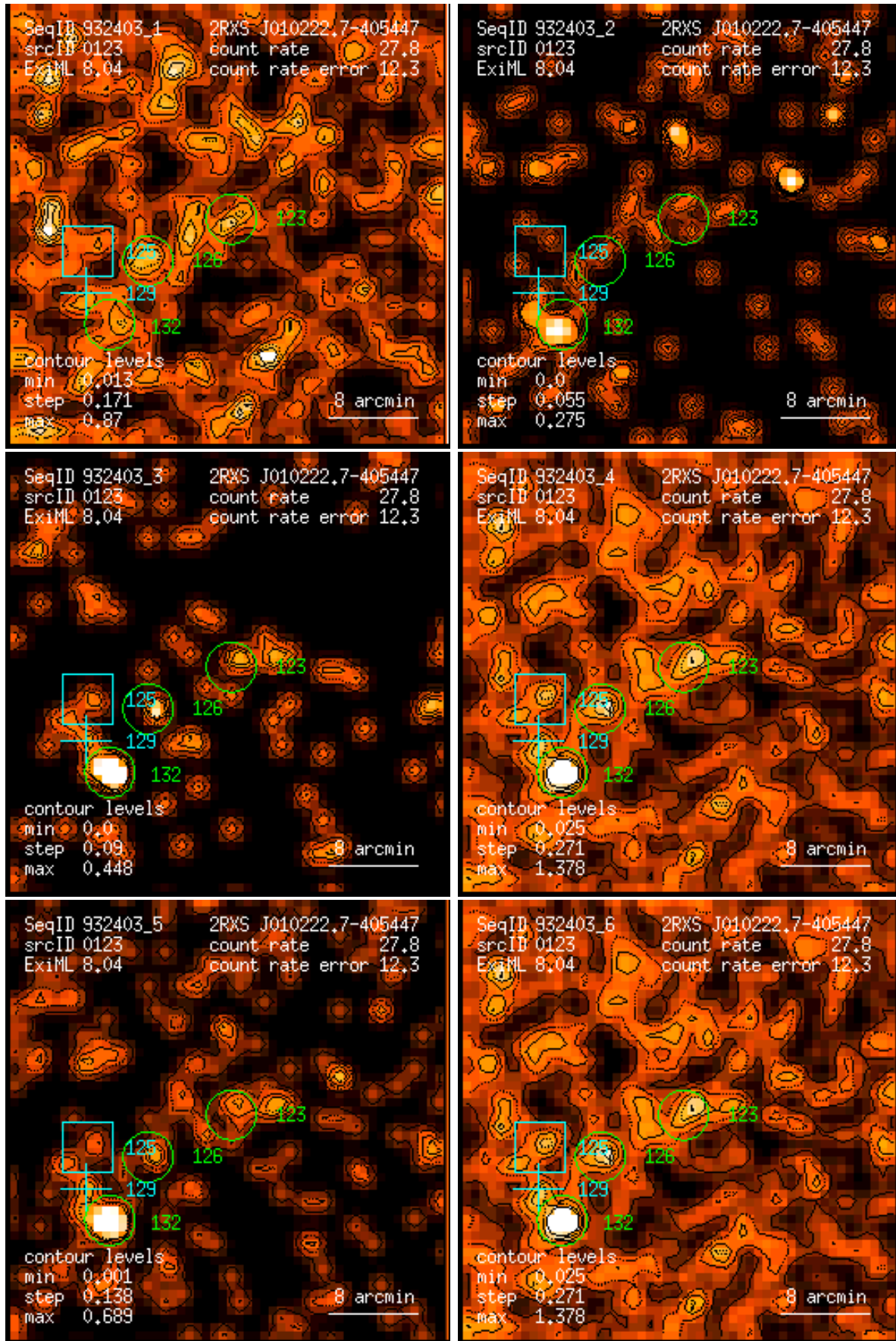
Figure 123: RASS 932403: detection 0123: band rate images, Gaussian filter: (1) PSPC channels 11 – 41, (2) 52 – 90, (3) 91 – 201, (4) 11 – 235, (5) 52 – 201, (6) 11 – 201. Broad band rates in counts/ks. Band rate contour levels in counts/ks/arcmin 2 .
