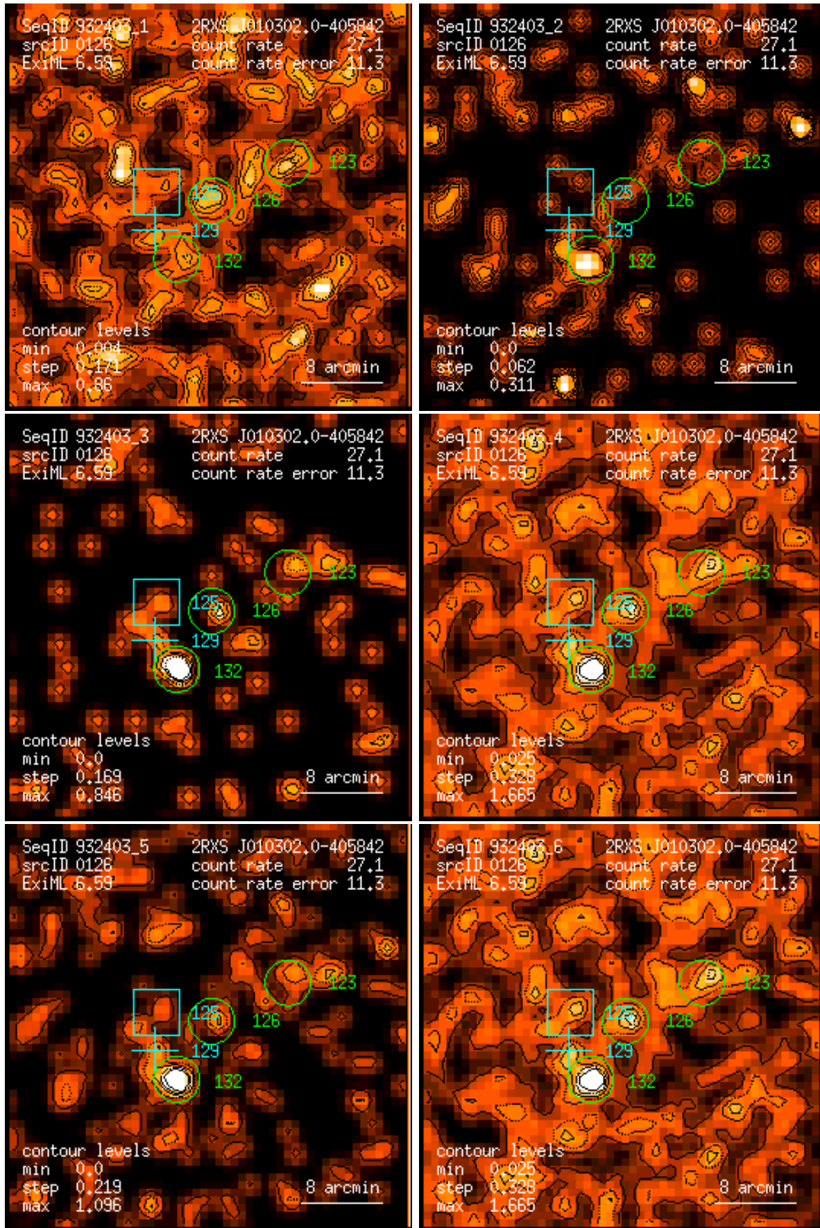
Figure 126: RASS 932403: detection 0126: band rate images, Gaussian filter: (1) PSPC channels 11 – 41, (2) 52 – 90, (3) 91 – 201, (4) 11 – 235, (5) 52 – 201, (6) 11 – 201. Broad band rates in counts/ks. Band rate contour levels in counts/ks/arcmin 2 .
