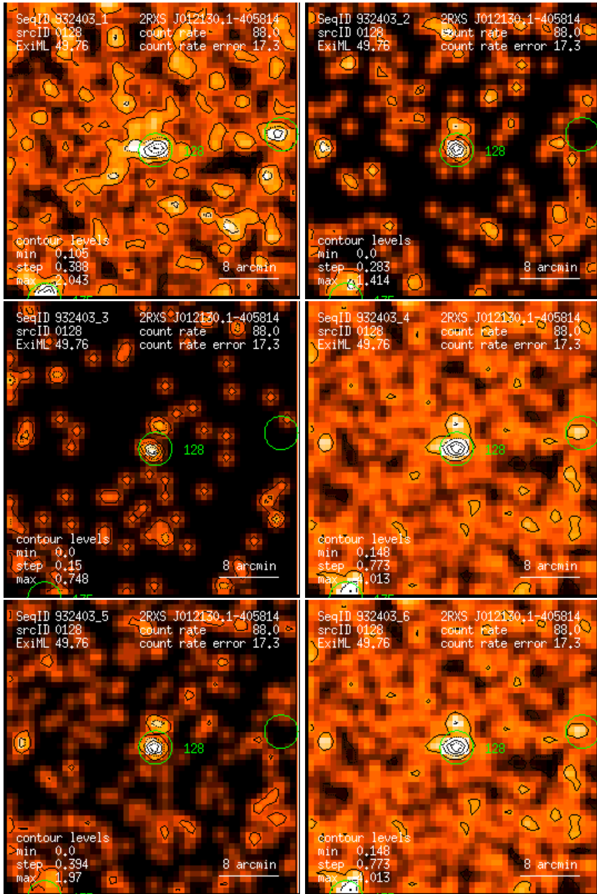
Figure 128: RASS 932403: detection 0128: band rate images, Gaussian filter: (1) PSPC channels 11 – 41, (2) 52 – 90, (3) 91 – 201, (4) 11 – 235, (5) 52 – 201, (6) 11 – 201. Broad band rates in counts/ks. Band rate contour levels in counts/ks/arcmin 2 .
