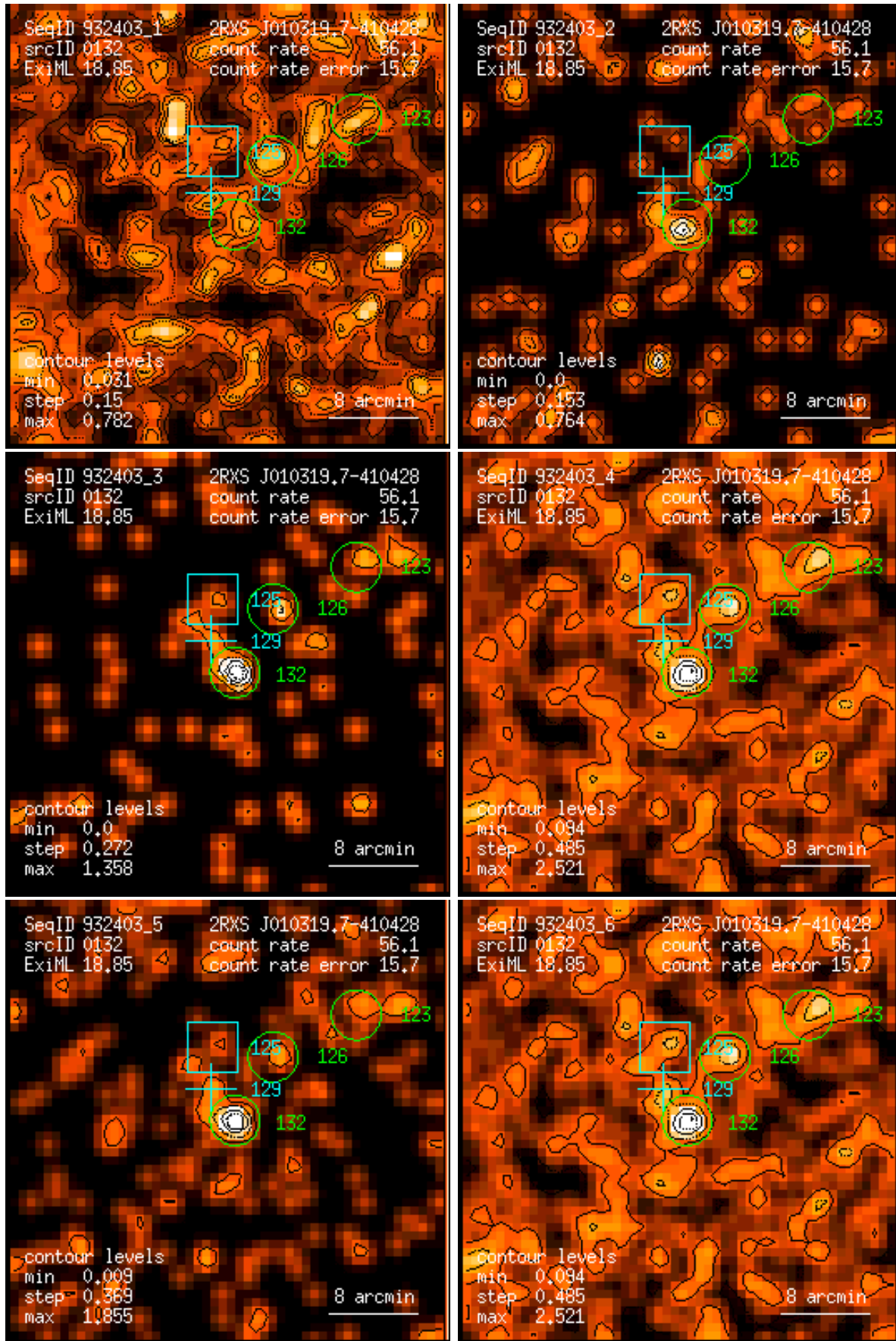
Figure 132: RASS 932403: detection 0132: band rate images, Gaussian filter: (1) PSPC channels 11 – 41, (2) 52 – 90, (3) 91 – 201, (4) 11 – 235, (5) 52 – 201, (6) 11 – 201. Broad band rates in counts/ks. Band rate contour levels in counts/ks/arcmin 2 .
