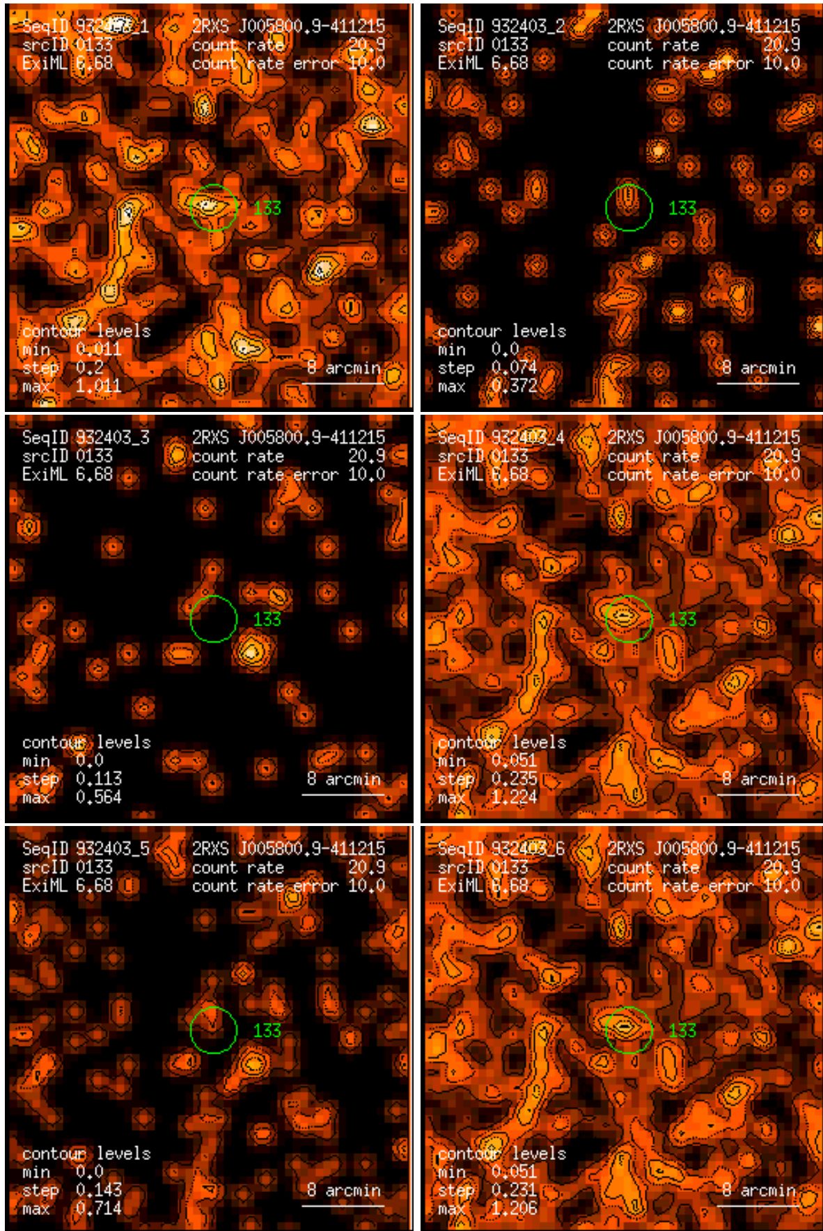
Figure 133: RASS 932403: detection 0133: band rate images, Gaussian filter: (1) PSPC channels 11 – 41, (2) 52 – 90, (3) 91 – 201, (4) 11 – 235, (5) 52 – 201, (6) 11 – 201. Broad band rates in counts/ks. Band rate contour levels in counts/ks/arcmin 2 .
