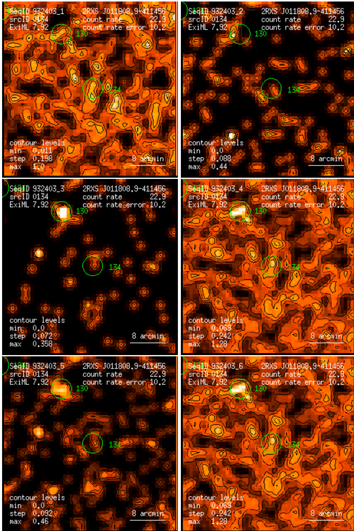
Figure 134: RASS 932403: detection 0134: band rate images, Gaussian filter: (1) PSPC channels 11 – 41, (2) 52 – 90, (3) 91 – 201, (4) 11 – 235, (5) 52 – 201, (6) 11 – 201. Broad band rates in counts/ks. Band rate contour levels in counts/ks/arcmin 2 .
