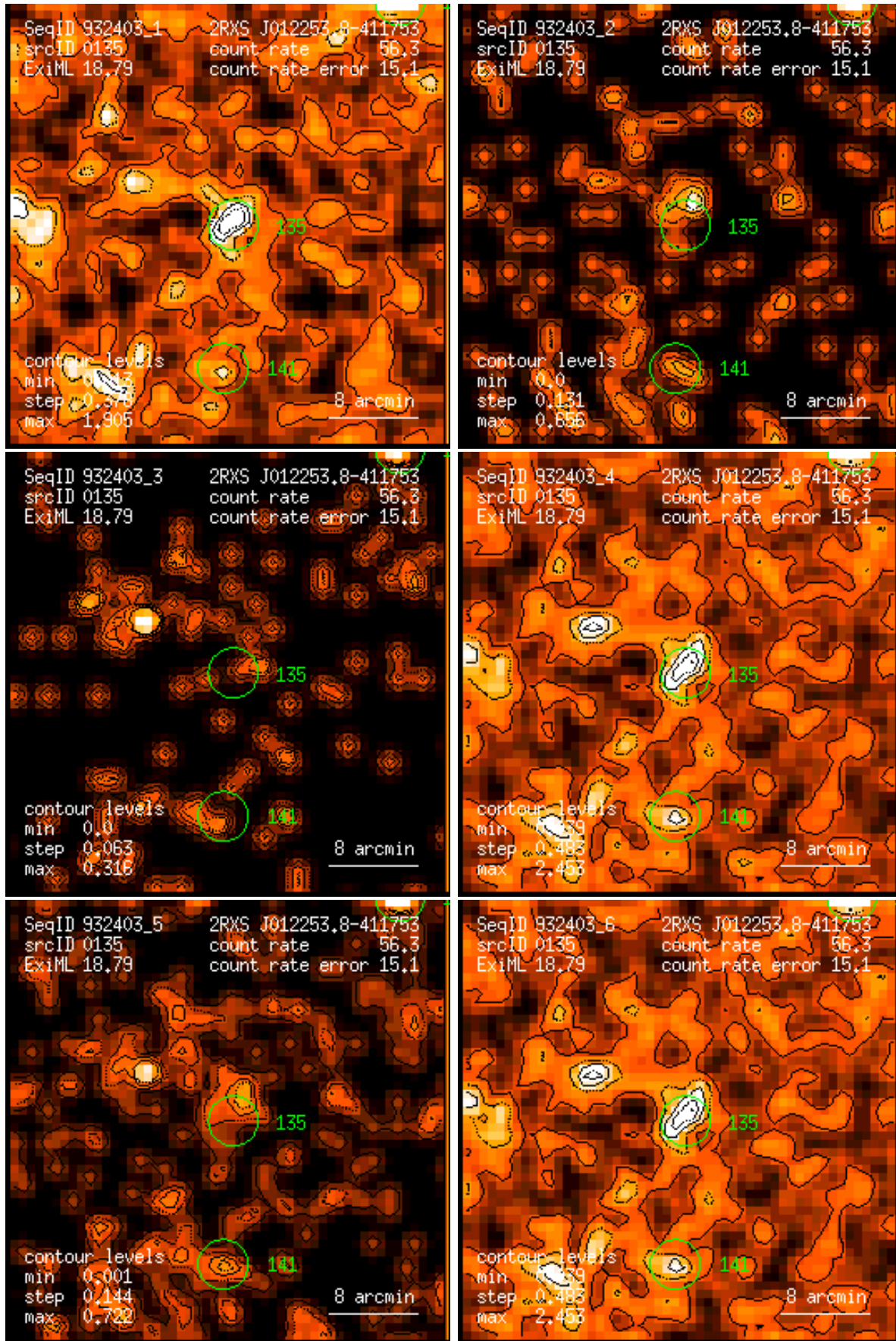
Figure 135: RASS 932403: detection 0135: band rate images, Gaussian filter: (1) PSPC channels 11 – 41, (2) 52 – 90, (3) 91 – 201, (4) 11 – 235, (5) 52 – 201, (6) 11 – 201. Broad band rates in counts/ks. Band rate contour levels in counts/ks/arcmin 2 .
