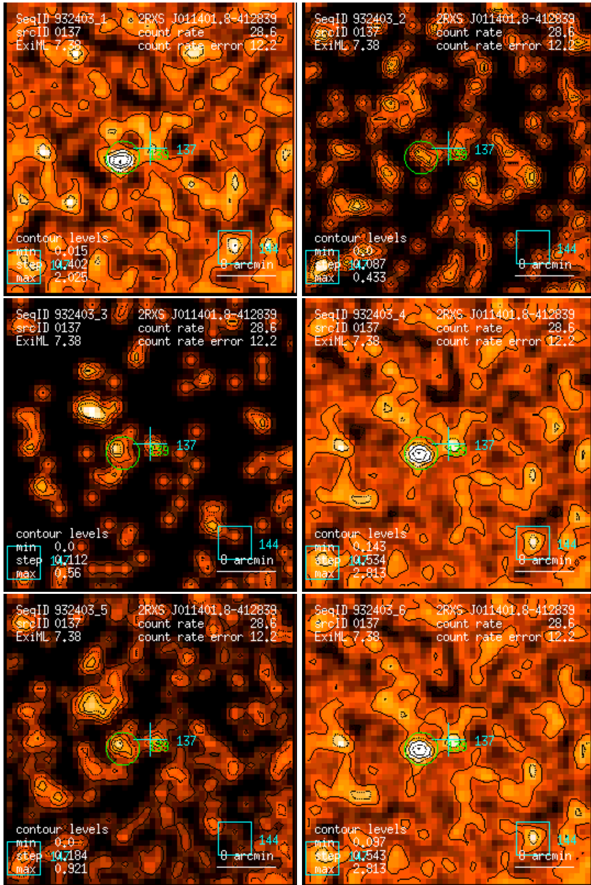
Figure 137: RASS 932403: detection 0137: band rate images, Gaussian filter: (1) PSPC channels 11 – 41, (2) 52 – 90, (3) 91 – 201, (4) 11 – 235, (5) 52 – 201, (6) 11 – 201. Broad band rates in counts/ks. Band rate contour levels in counts/ks/arcmin 2 .
