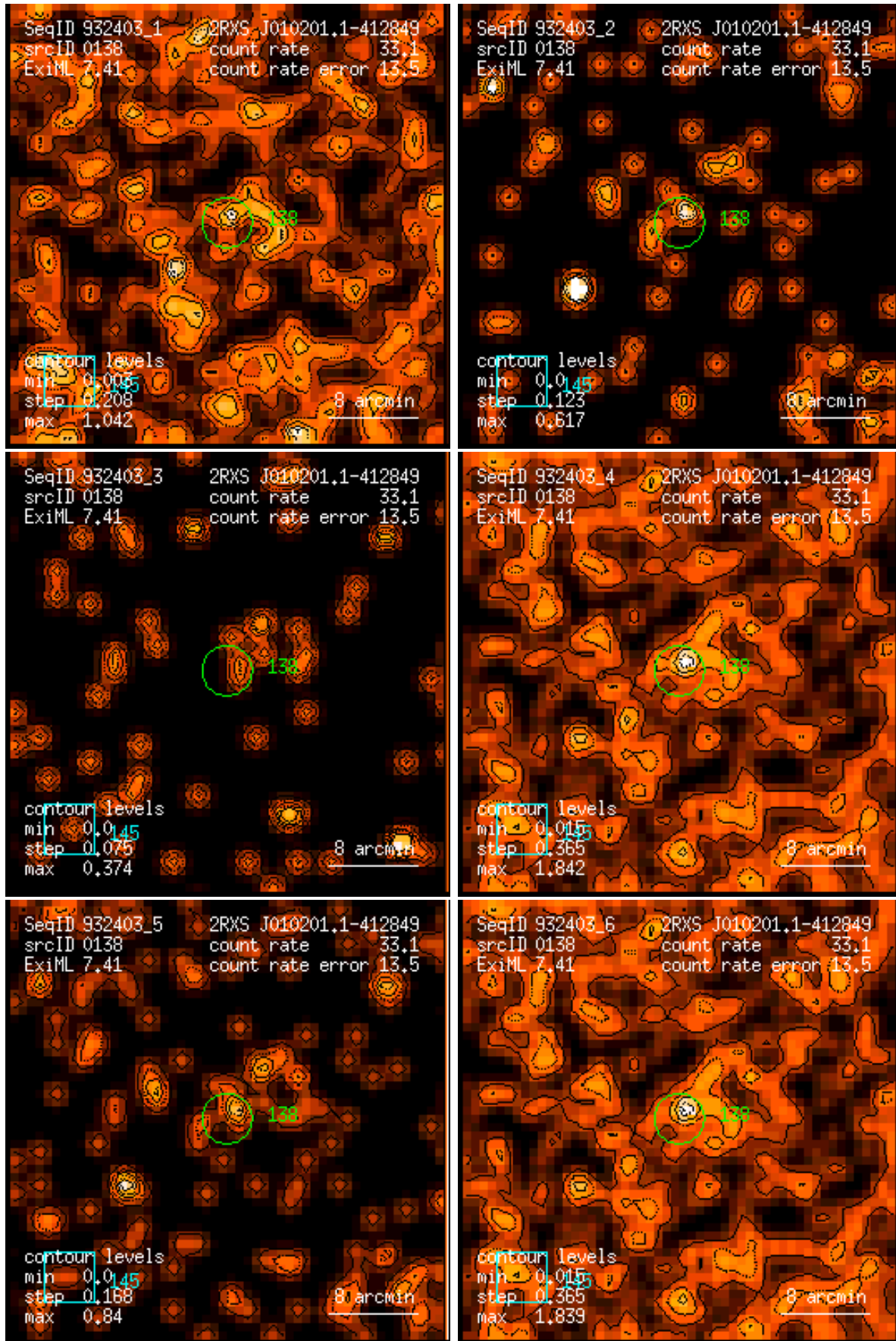
Figure 138: RASS 932403: detection 0138: band rate images, Gaussian filter: (1) PSPC channels 11 – 41, (2) 52 – 90, (3) 91 – 201, (4) 11 – 235, (5) 52 – 201, (6) 11 – 201. Broad band rates in counts/ks. Band rate contour levels in counts/ks/arcmin 2 .
