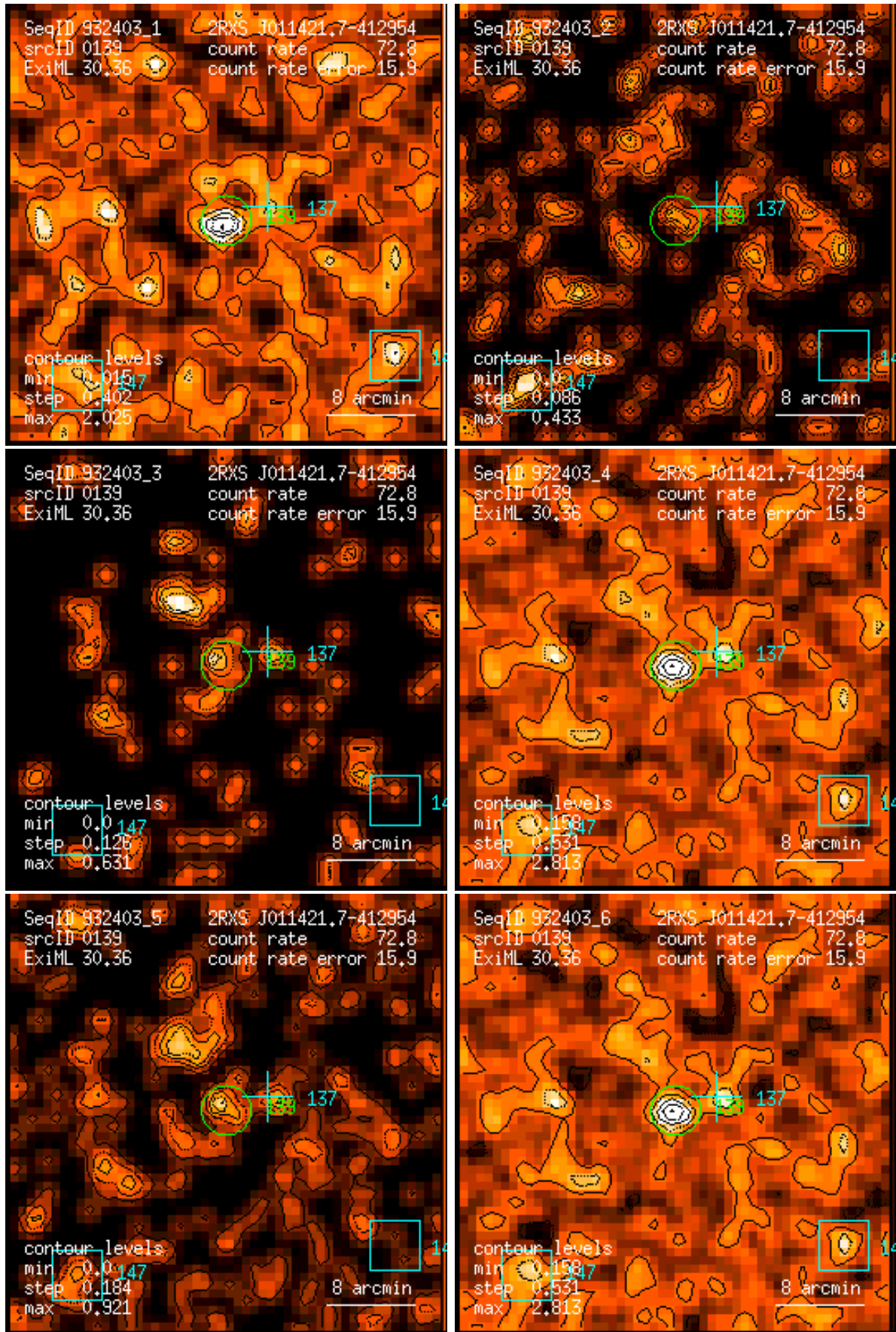
Figure 139: RASS 932403: detection 0139: band rate images, Gaussian filter: (1) PSPC channels 11 – 41, (2) 52 – 90, (3) 91 – 201, (4) 11 – 235, (5) 52 – 201, (6) 11 – 201. Broad band rates in counts/ks. Band rate contour levels in counts/ks/arcmin 2 .
