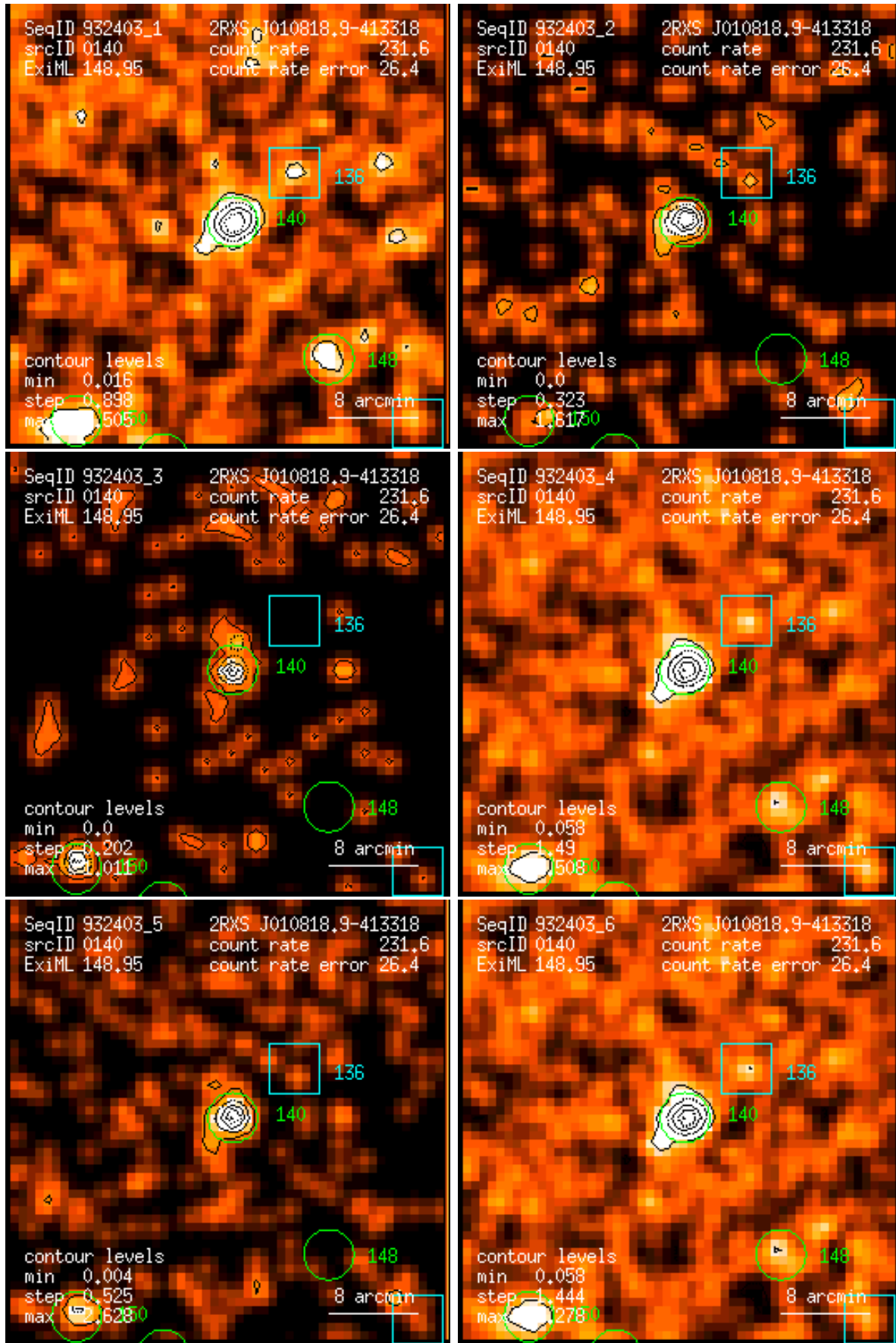
Figure 140: RASS 932403: detection 0140: band rate images, Gaussian filter: (1) PSPC channels 11 – 41, (2) 52 – 90, (3) 91 – 201, (4) 11 – 235, (5) 52 – 201, (6) 11 – 201. Broad band rates in counts/ks. Band rate contour levels in counts/ks/arcmin 2 .
