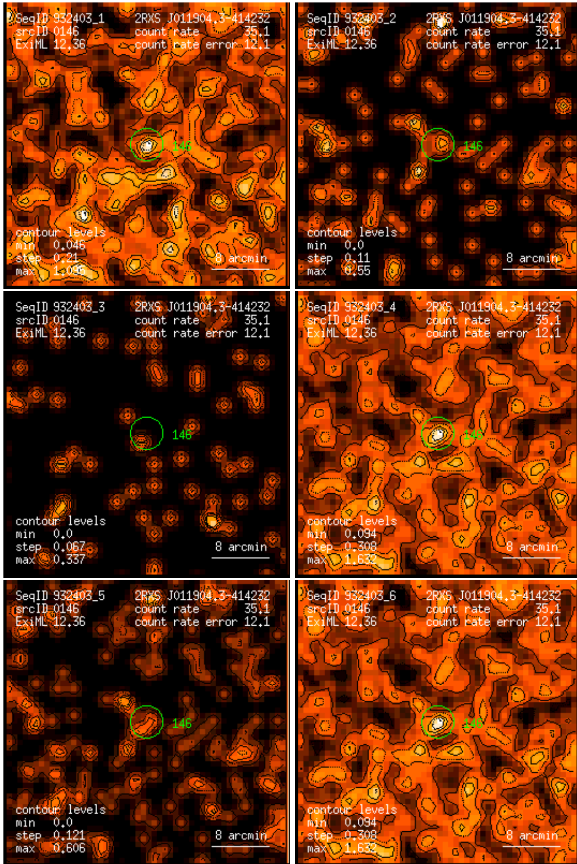
Figure 146: RASS 932403: detection 0146: band rate images, Gaussian filter: (1) PSPC channels 11 – 41, (2) 52 – 90, (3) 91 – 201, (4) 11 – 235, (5) 52 – 201, (6) 11 – 201. Broad band rates in counts/ks. Band rate contour levels in counts/ks/arcmin 2 .
