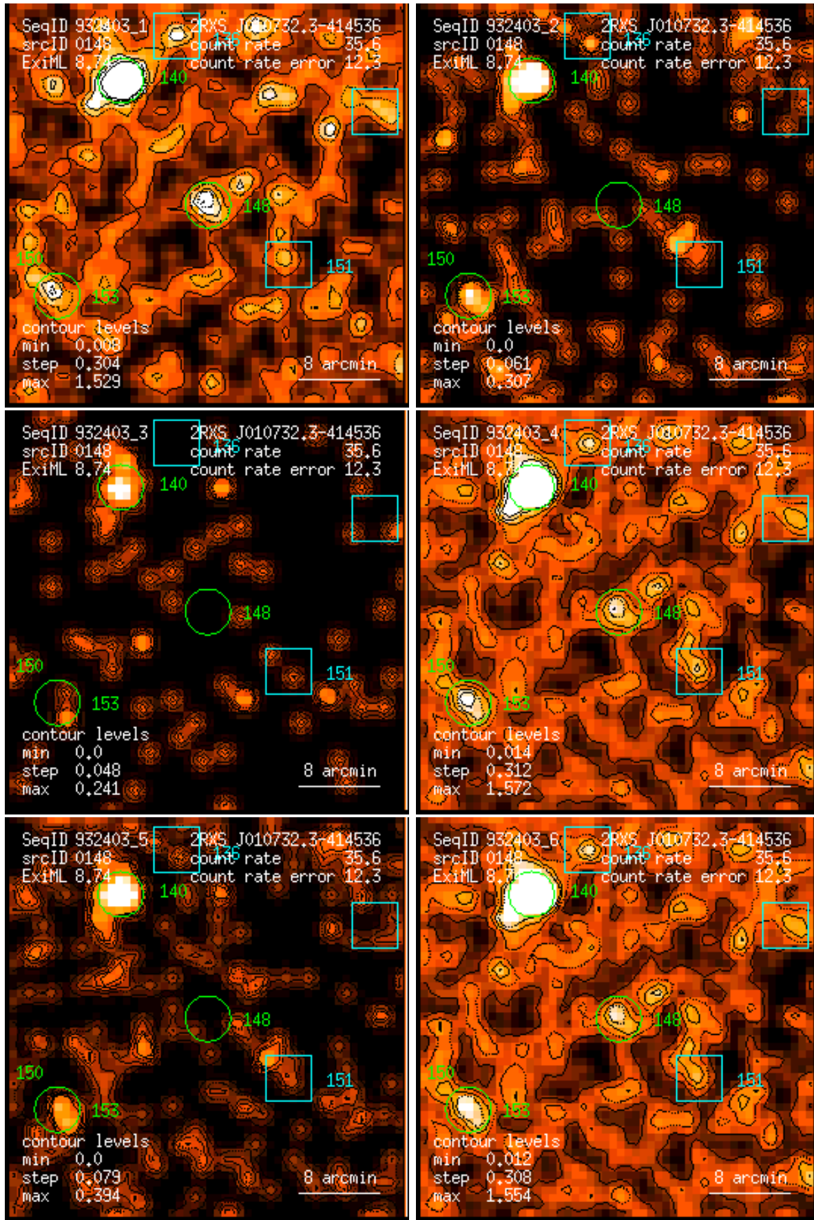
Figure 148: RASS 932403: detection 0148: band rate images, Gaussian filter: (1) PSPC channels 11 – 41, (2) 52 – 90, (3) 91 – 201, (4) 11 – 235, (5) 52 – 201, (6) 11 – 201. Broad band rates in counts/ks. Band rate contour levels in counts/ks/arcmin 2 .
