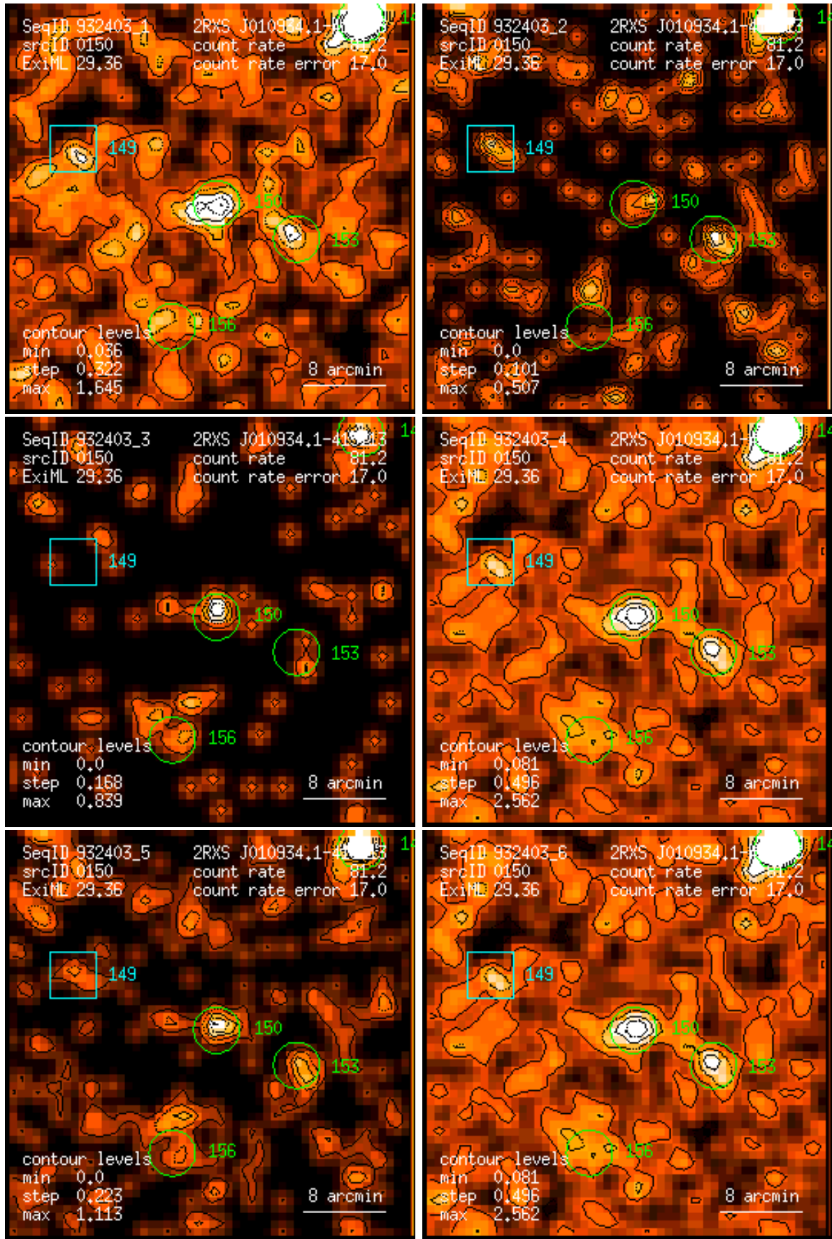
Figure 150: RASS 932403: detection 0150: band rate images, Gaussian filter: (1) PSPC channels 11 – 41, (2) 52 – 90, (3) 91 – 201, (4) 11 – 235, (5) 52 – 201, (6) 11 – 201. Broad band rates in counts/ks. Band rate contour levels in counts/ks/arcmin 2 .
