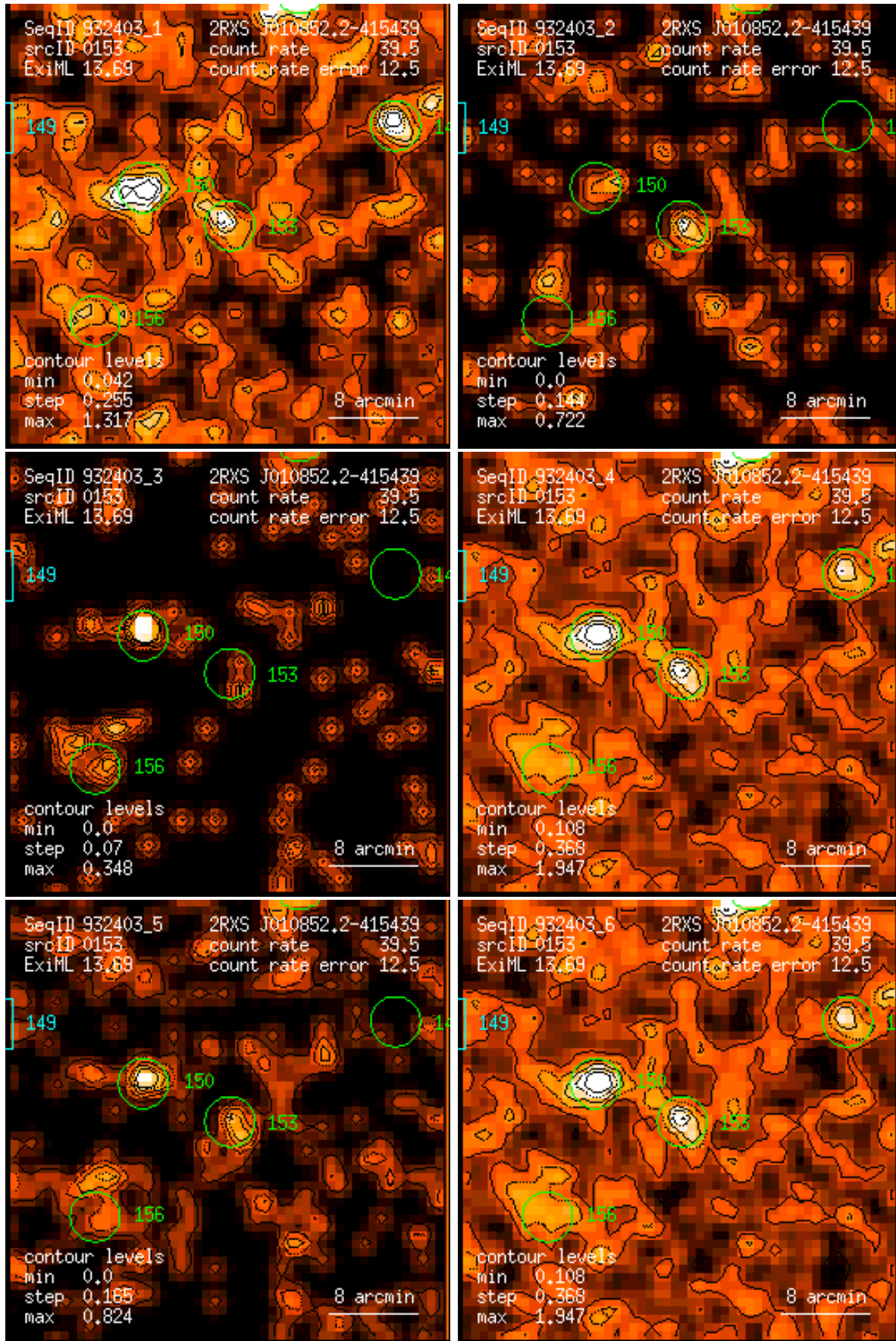
Figure 153: RASS 932403: detection 0153: band rate images, Gaussian filter: (1) PSPC channels 11 – 41, (2) 52 – 90, (3) 91 – 201, (4) 11 – 235, (5) 52 – 201, (6) 11 – 201. Broad band rates in counts/ks. Band rate contour levels in counts/ks/arcmin 2 .
