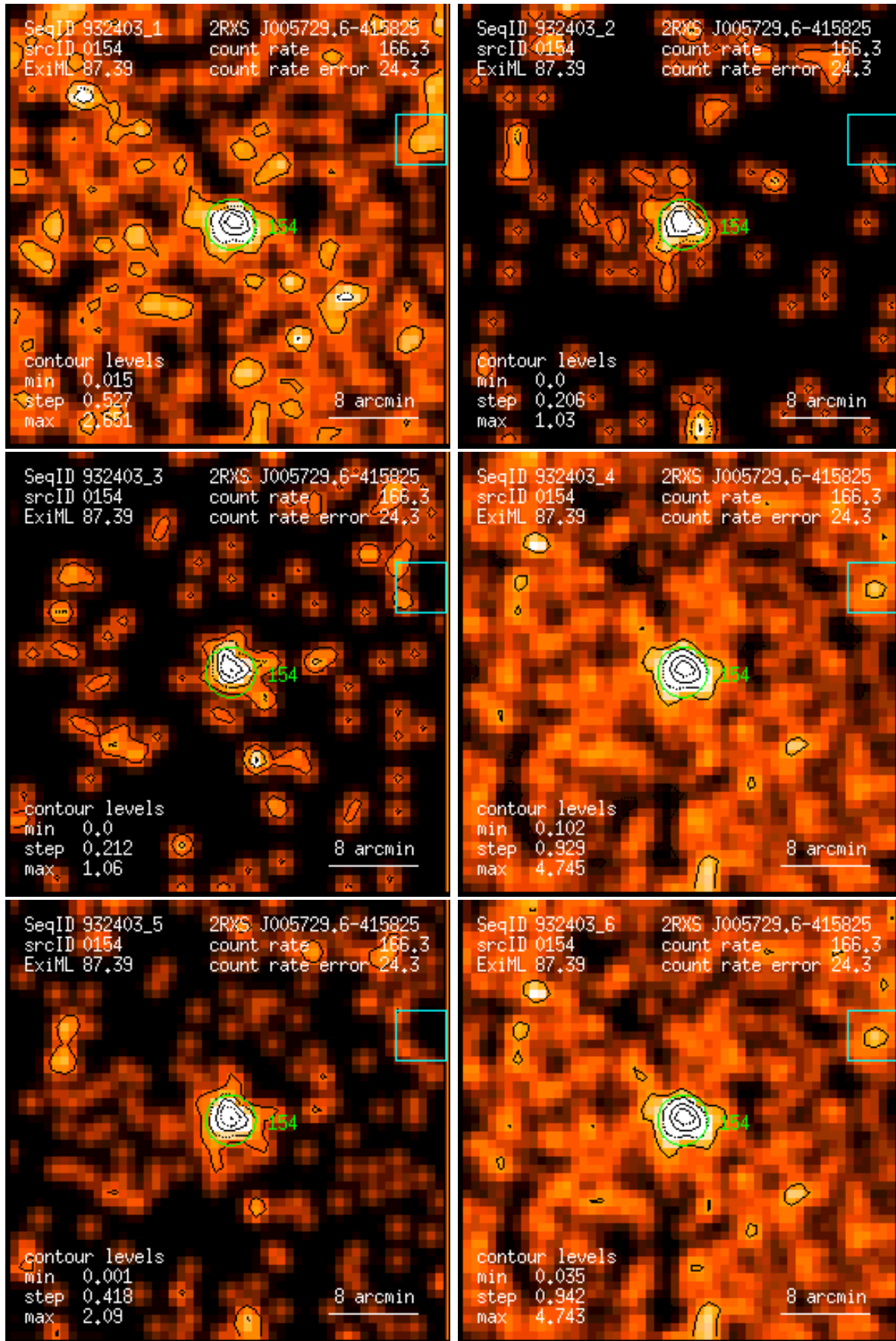
Figure 154: RASS 932403: detection 0154: band rate images, Gaussian filter: (1) PSPC channels 11 – 41, (2) 52 – 90, (3) 91 – 201, (4) 11 – 235, (5) 52 – 201, (6) 11 – 201. Broad band rates in counts/ks. Band rate contour levels in counts/ks/arcmin 2 .
