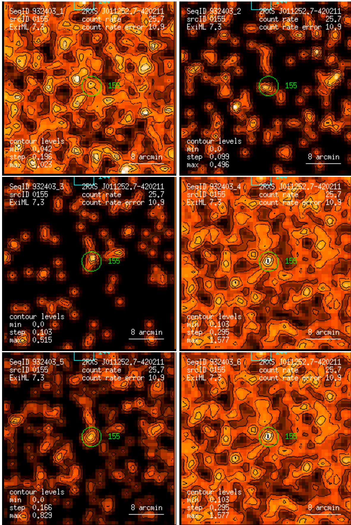
Figure 155: RASS 932403: detection 0155: band rate images, Gaussian filter: (1) PSPC channels 11 – 41, (2) 52 – 90, (3) 91 – 201, (4) 11 – 235, (5) 52 – 201, (6) 11 – 201. Broad band rates in counts/ks. Band rate contour levels in counts/ks/arcmin 2 .
