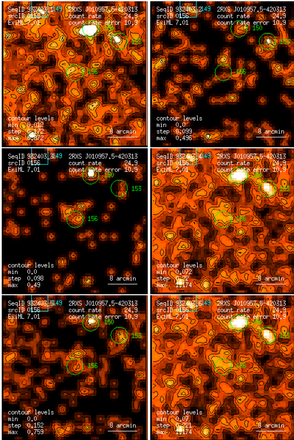
Figure 156: RASS 932403: detection 0156: band rate images, Gaussian filter: (1) PSPC channels 11 – 41, (2) 52 – 90, (3) 91 – 201, (4) 11 – 235, (5) 52 – 201, (6) 11 – 201. Broad band rates in counts/ks. Band rate contour levels in counts/ks/arcmin 2 .
