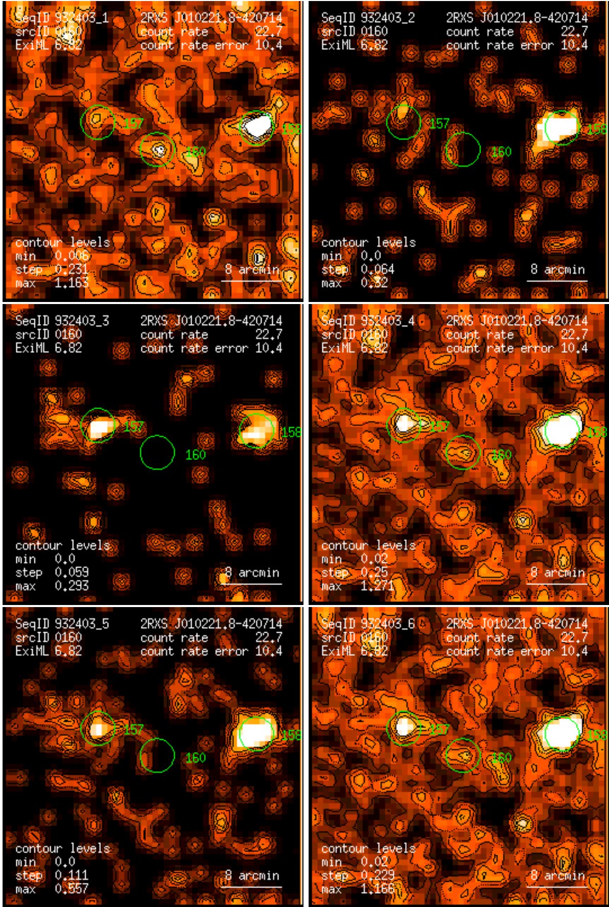
Figure 160: RASS 932403: detection 0160: band rate images, Gaussian filter: (1) PSPC channels 11 – 41, (2) 52 – 90, (3) 91 – 201, (4) 11 – 235, (5) 52 – 201, (6) 11 – 201. Broad band rates in counts/ks. Band rate contour levels in counts/ks/arcmin 2 .
