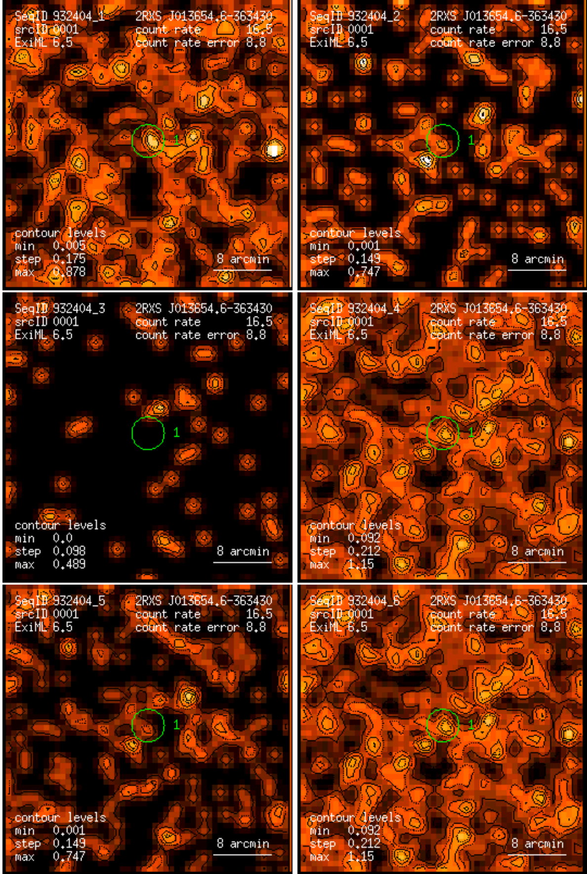
Figure 1: RASS 932404: detection 0001: band rate images, Gaussian filter: (1) PSPC channels 11 – 41, (2) 52 – 90, (3) 91 – 201, (4) 11 – 235, (5) 52 – 201, (6) 11 – 201. Broad band rates in counts/ks. Band rate contour levels in counts/ks/arcmin 2 .
