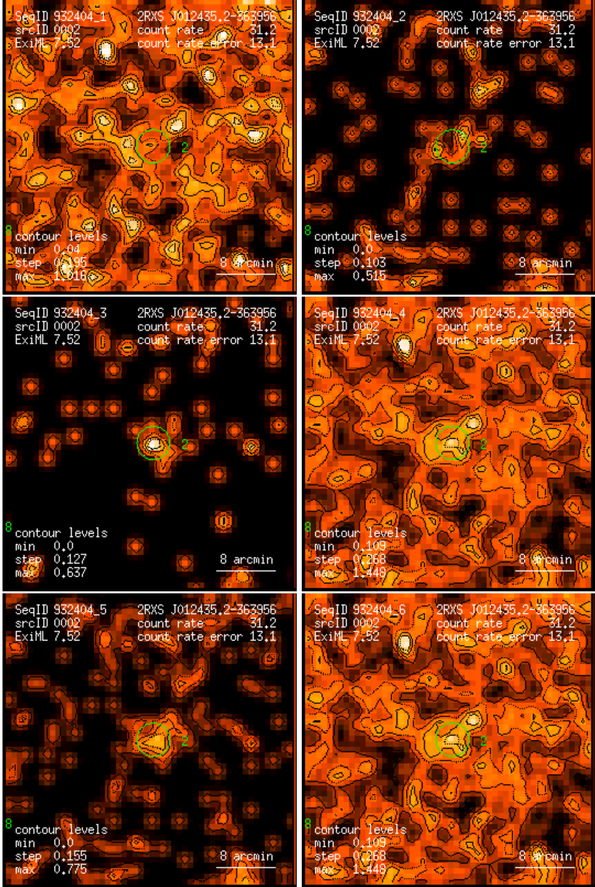
Figure 2: RASS 932404: detection 0002: band rate images, Gaussian filter: (1) PSPC channels 11 – 41, (2) 52 – 90, (3) 91 – 201, (4) 11 – 235, (5) 52 – 201, (6) 11 – 201. Broad band rates in counts/ks. Band rate contour levels in counts/ks/arcmin 2 .
