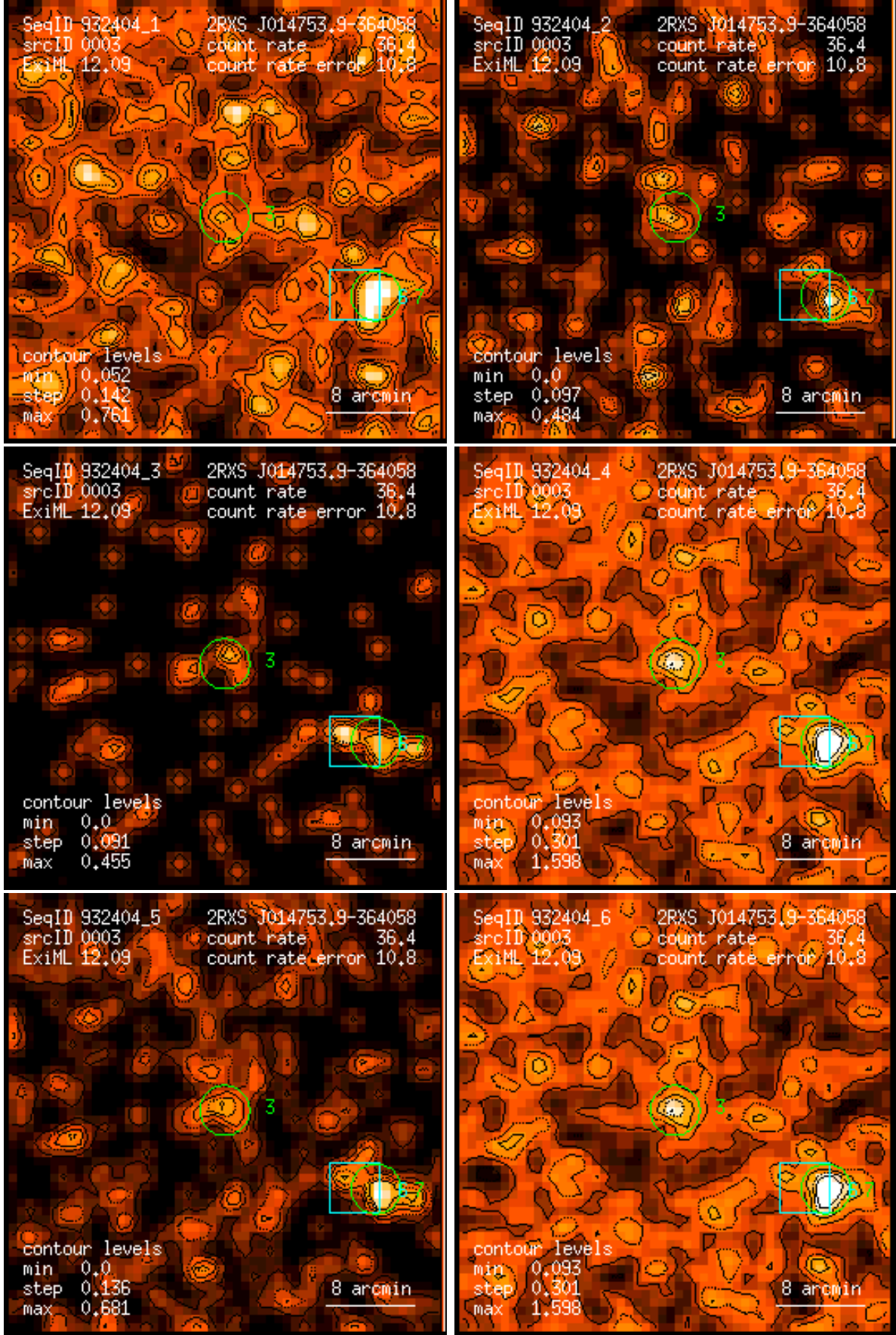
Figure 3: RASS 932404: detection 0003: band rate images, Gaussian filter: (1) PSPC channels 11 – 41, (2) 52 – 90, (3) 91 – 201, (4) 11 – 235, (5) 52 – 201, (6) 11 – 201. Broad band rates in counts/ks. Band rate contour levels in counts/ks/arcmin 2 .
