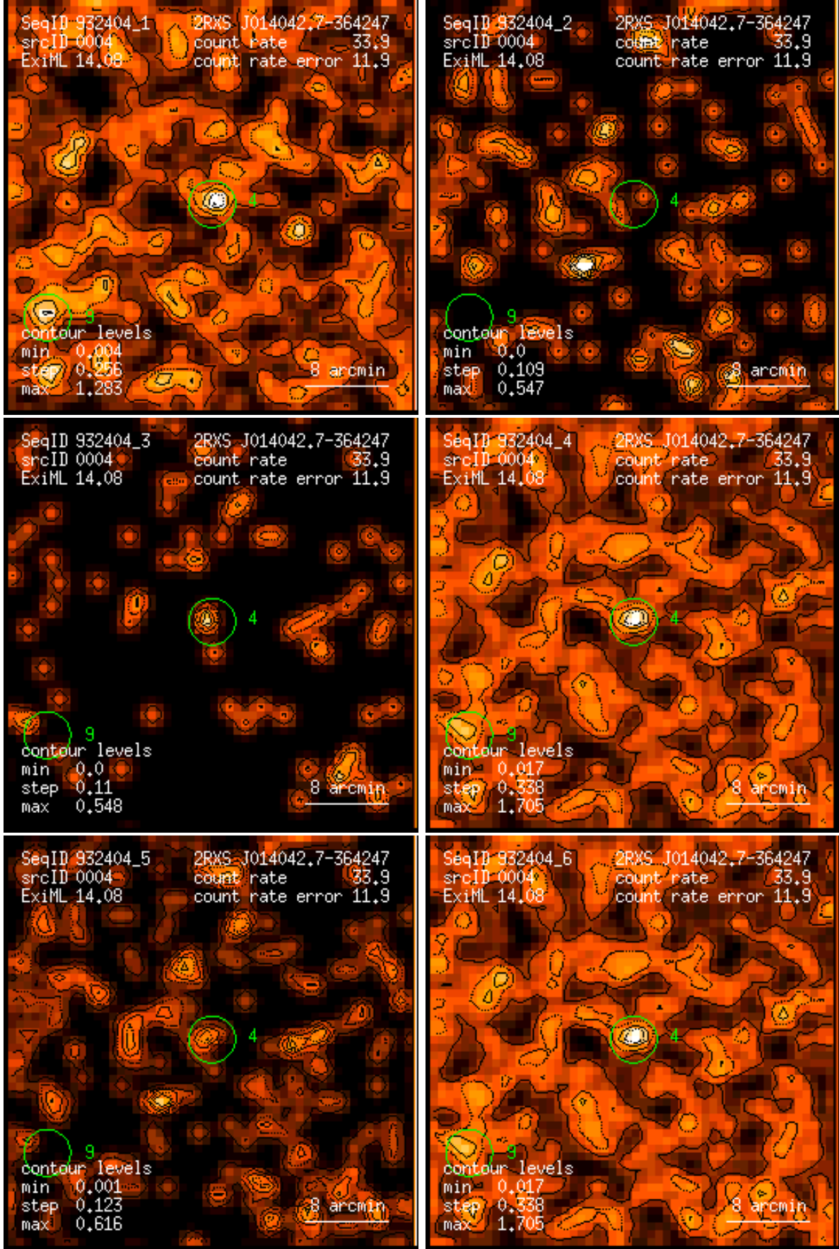
Figure 4: RASS 932404: detection 0004: band rate images, Gaussian filter: (1) PSPC channels 11 – 41, (2) 52 – 90, (3) 91 – 201, (4) 11 – 235, (5) 52 – 201, (6) 11 – 201. Broad band rates in counts/ks. Band rate contour levels in counts/ks/arcmin 2 .
