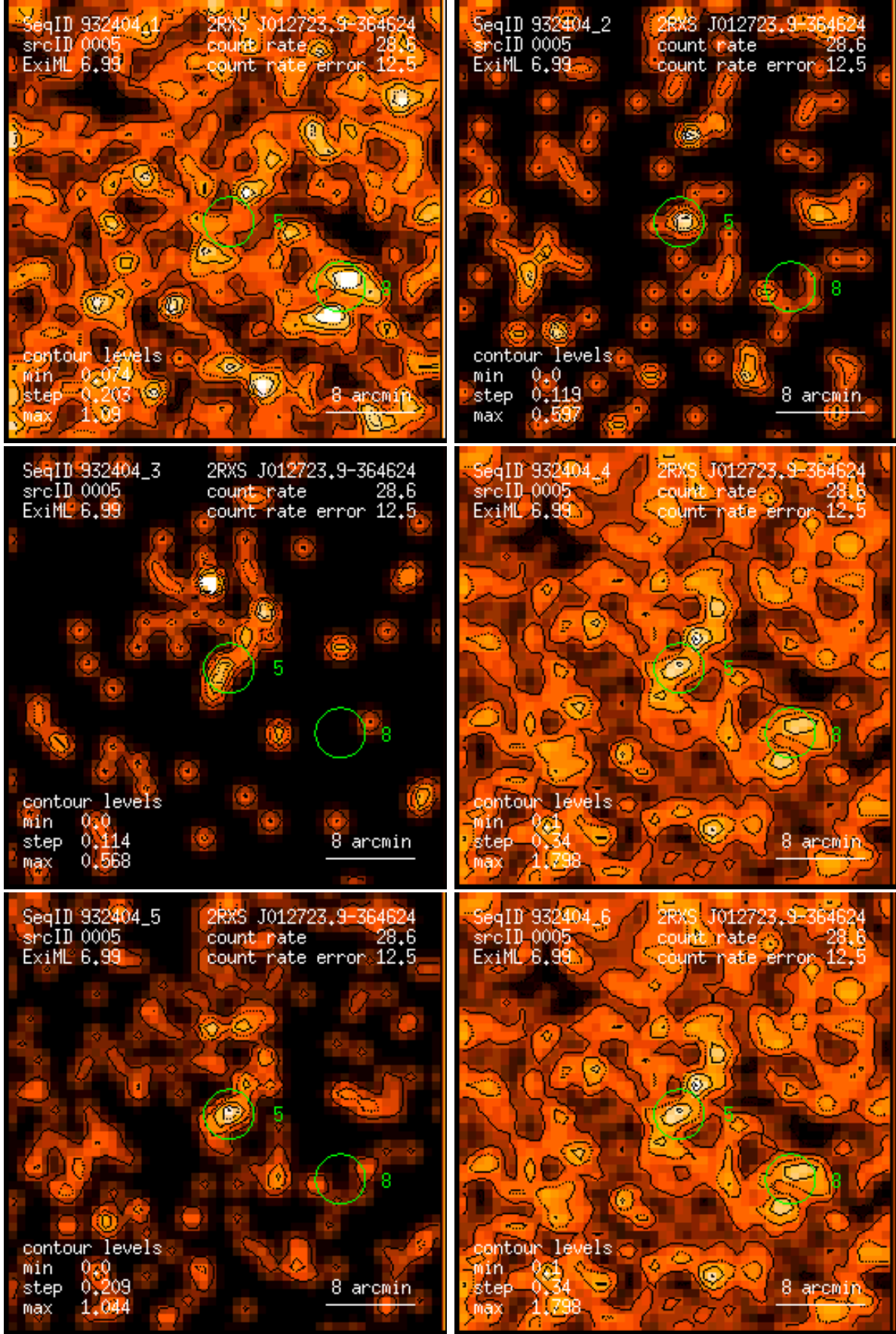
Figure 5: RASS 932404: detection 0005: band rate images, Gaussian filter: (1) PSPC channels 11 – 41, (2) 52 – 90, (3) 91 – 201, (4) 11 – 235, (5) 52 – 201, (6) 11 – 201. Broad band rates in counts/ks. Band rate contour levels in counts/ks/arcmin 2 .
