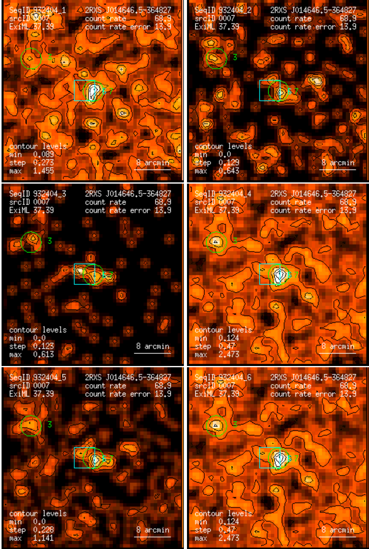
Figure 7: RASS 932404: detection 0007: band rate images, Gaussian filter: (1) PSPC channels 11 – 41, (2) 52 – 90, (3) 91 – 201, (4) 11 – 235, (5) 52 – 201, (6) 11 – 201. Broad band rates in counts/ks. Band rate contour levels in counts/ks/arcmin 2 .
